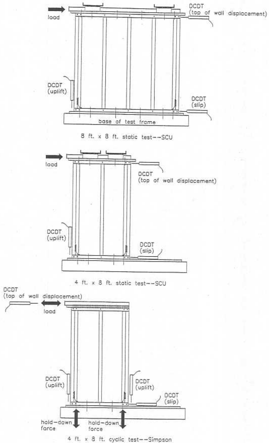
Figure 4 Instrumentation for static and cyclic tests
