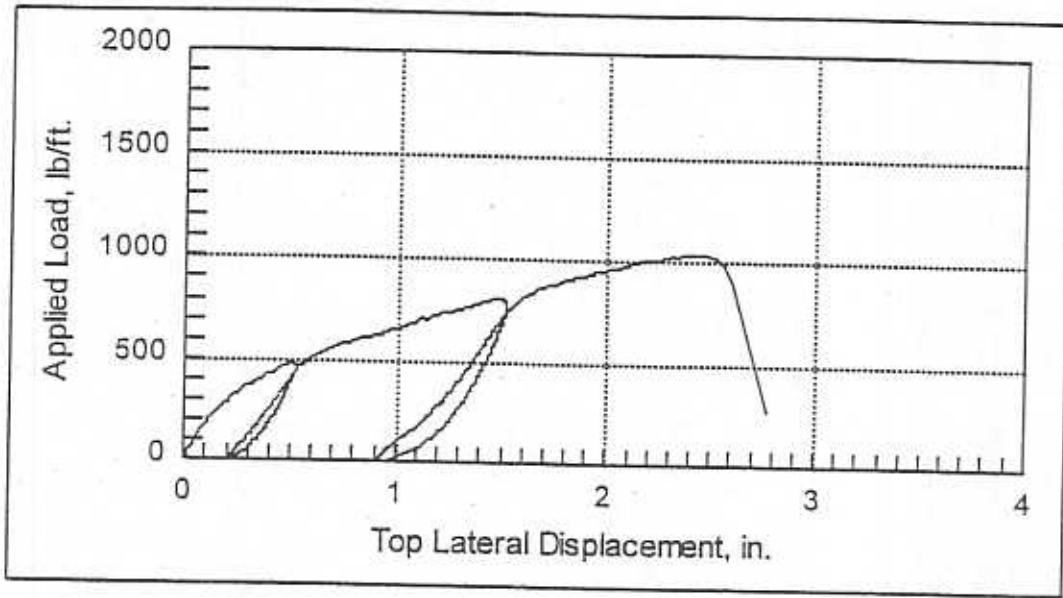
Fig. 1 Load vs. top of wall lateral displacement for specimen PLY-1A6
