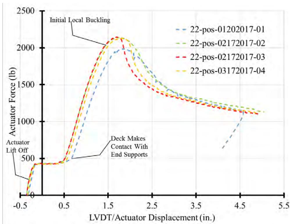
Figure 73: Overlay of 22 Gage Positive Test Results.
