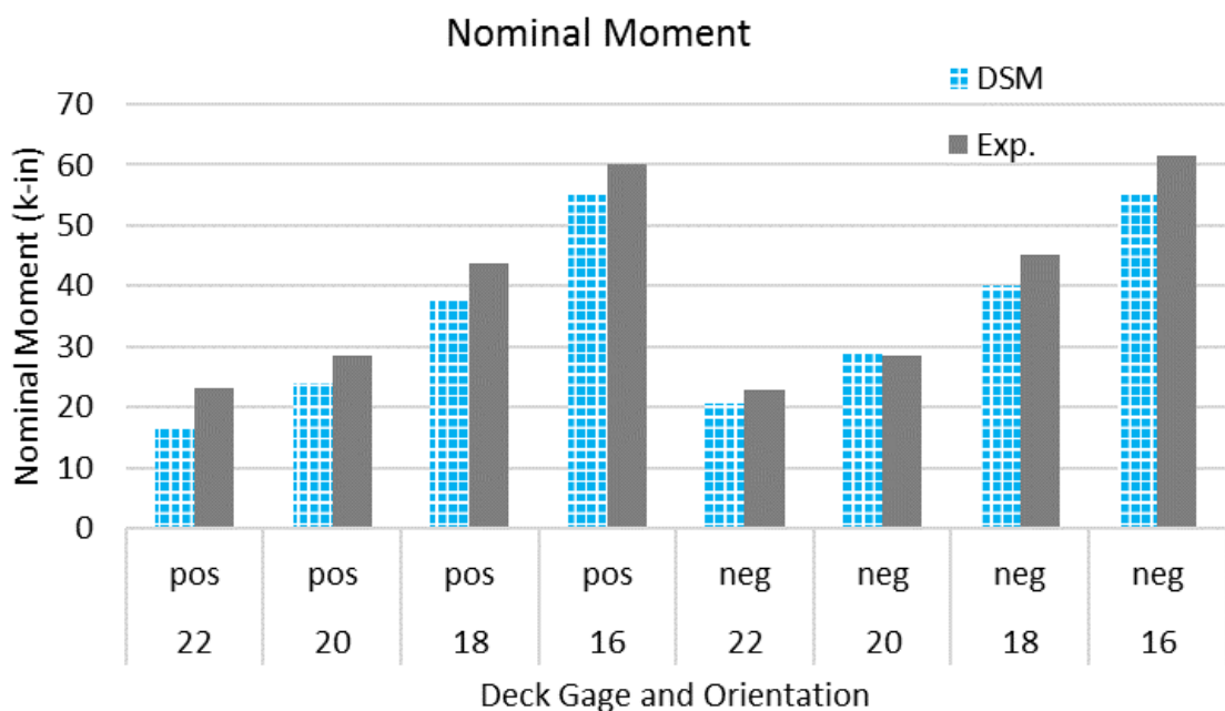
Figure 78: DSM Nominal Moment versus Experimental Nominal Moment.
