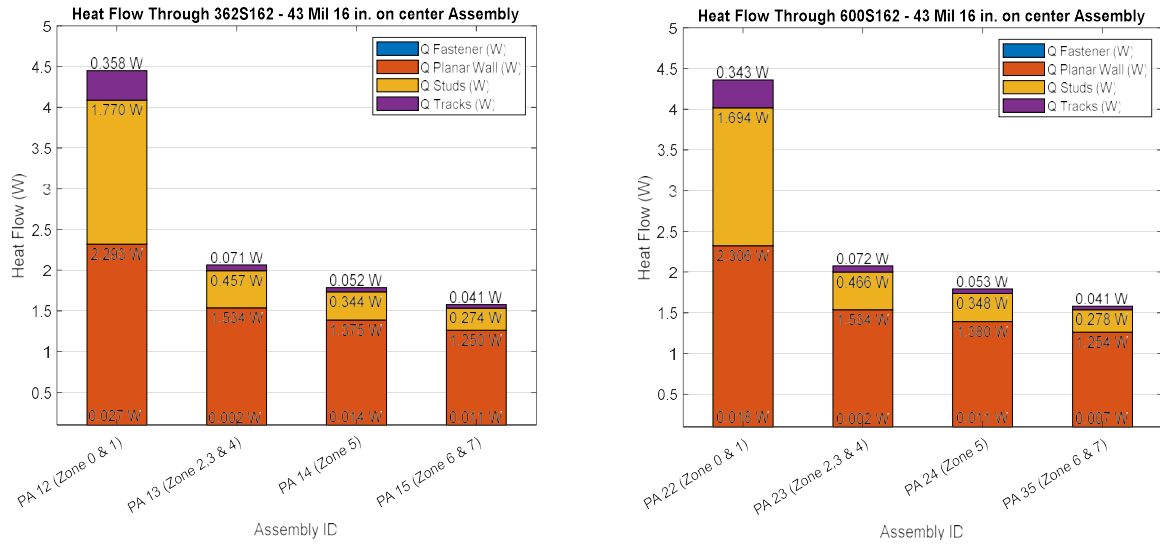
Figure 15: Comparison of Heat Flow through 362S162 - 43 Mil 16 in. on center and 600S162 - 43 mil 16 in. on center Assemblies
