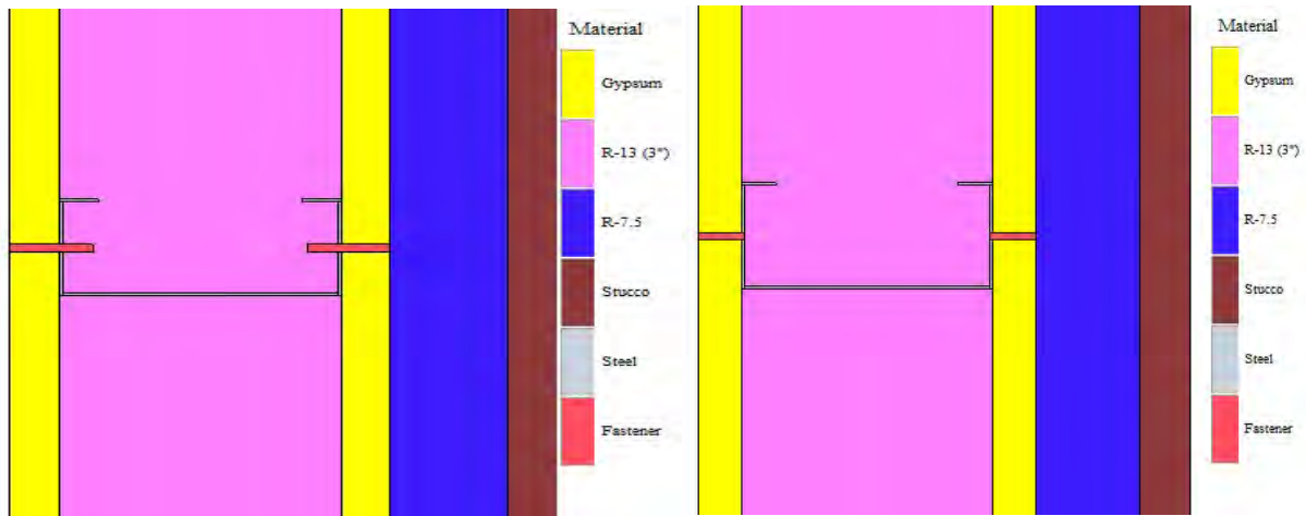
Figure 11: 2-D Section Cut through Wall Assembly at Fastener Locations (Left – Fastener length modelled and Right – Fastener modelled from start of sheathing to interior of Flange)
