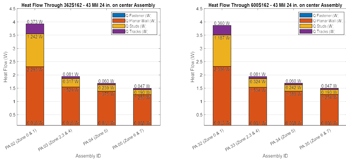
Figure 14: Comparison of Heat Flow through 362S162 - 43 Mil 24 in. on center and 600S162 - 43 mil 24 in. on center Assemblies
