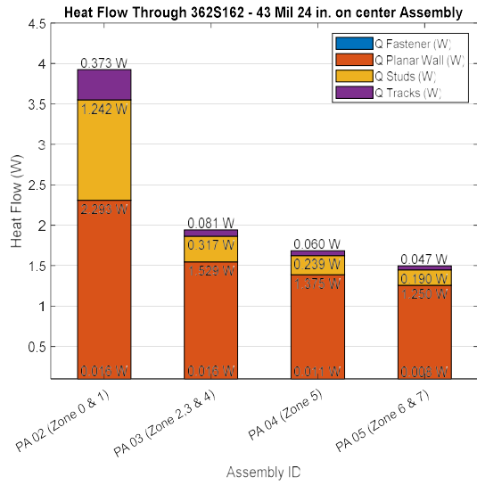
Figure 18: Comparison of Heat Flow through 362S162 - 43 Mil 24 in. on center and 362S162 - 43 Mil 16 in. on center Assemblies
