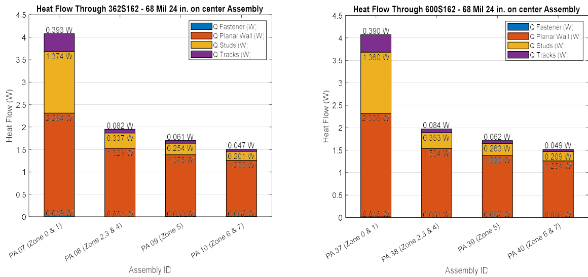
Figure 16: Comparison of Heat Flow through 362S162 - 68 Mil 24 in. on center and 600S162 - 68 mil 24 in. on center Assemblies
