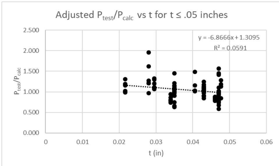
Figure 4.7 Adjusted P_{test}/P_{calc} versus t for t \leq 0.05 inches
