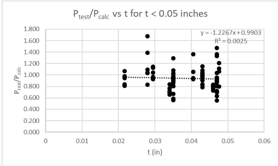
Figure 4.6 Original P_{test}/P_{calc} versus t for t \leq 0.05 inches
