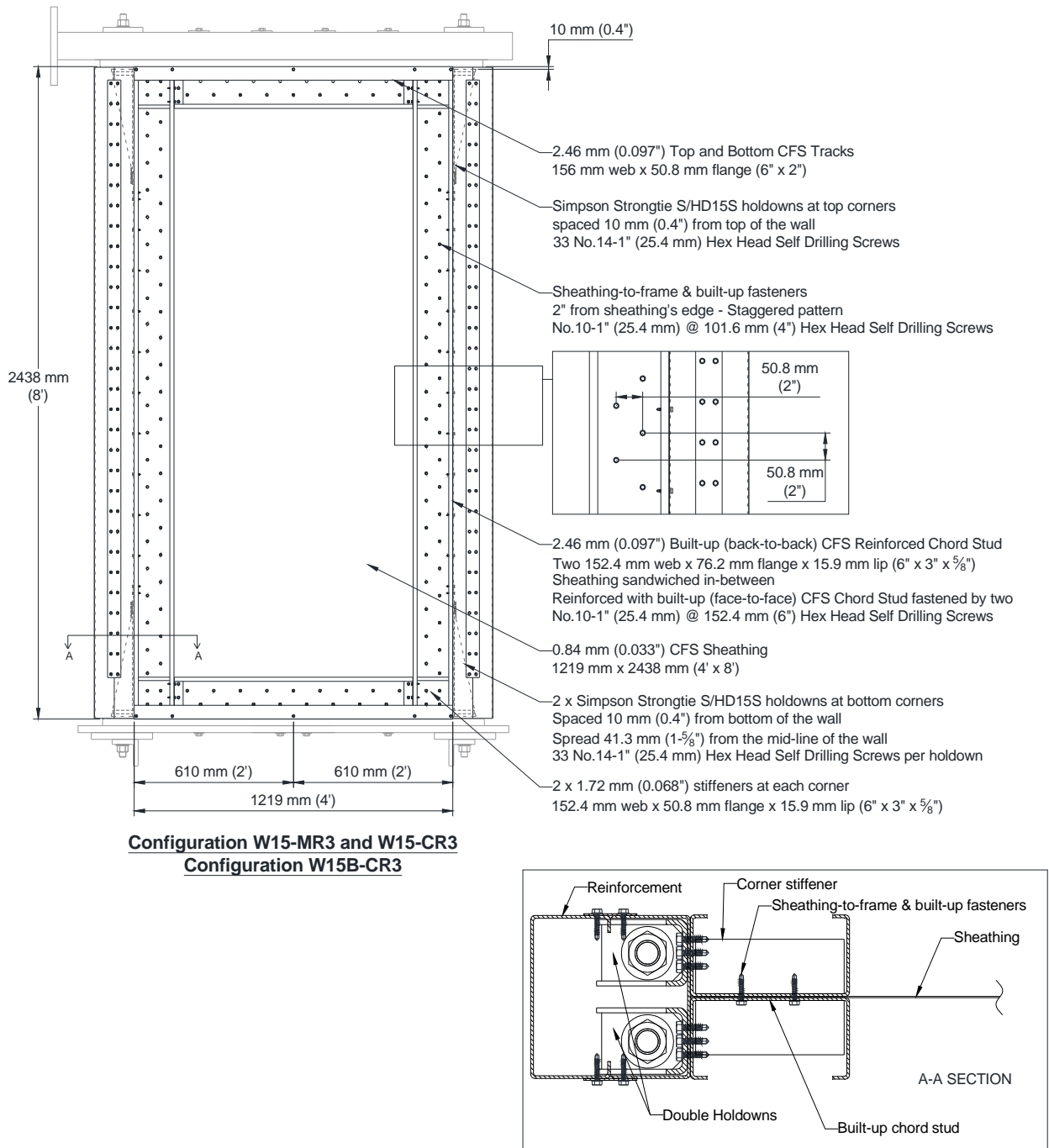
Figure A6: Nominal dimensions and specifications of specimens W15-MR3, W15-CR3, and W15B-CR3.
