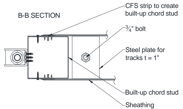
Figure A5: Double-sheathed configuration cross-section details.
