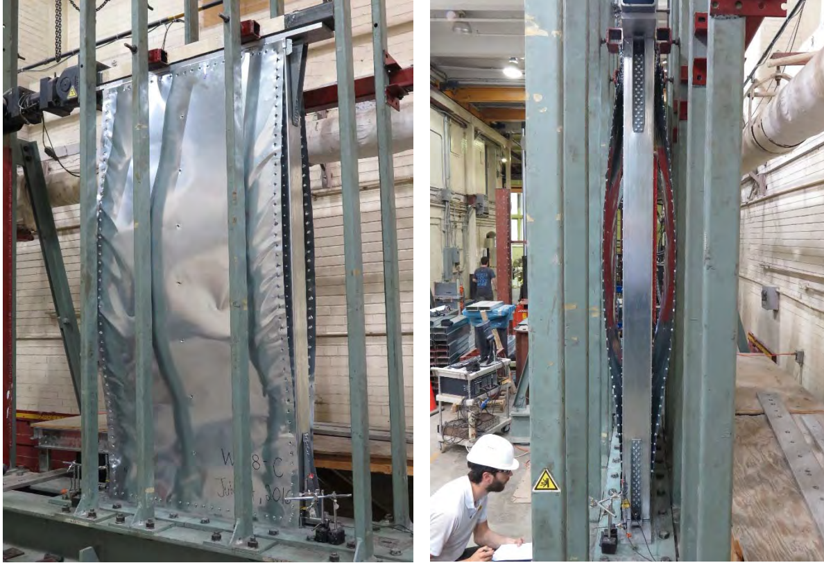
Figure 2.4: Sheathing detached from double-sheathed shear wall subjected to reversed cyclic loading.
