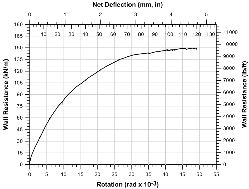
Figure E9: Monotonic test data of centre-sheathed specimen W15-MR3.
