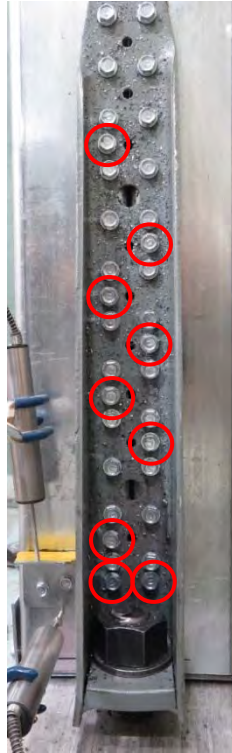
Figure 2.17: Extra holddown screws holes (circled in red) drilled to accommodate for the sheathing in the centre.
