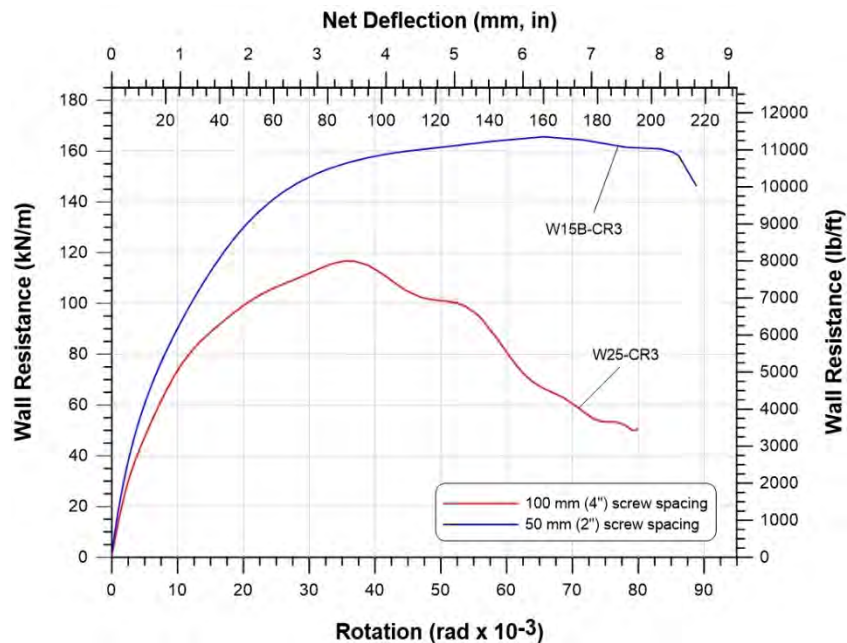
Figure 3.25: Comparison of sheathing fastener spacing between centre-sheathed specimens W15B-CR3 and W25-CR3.
