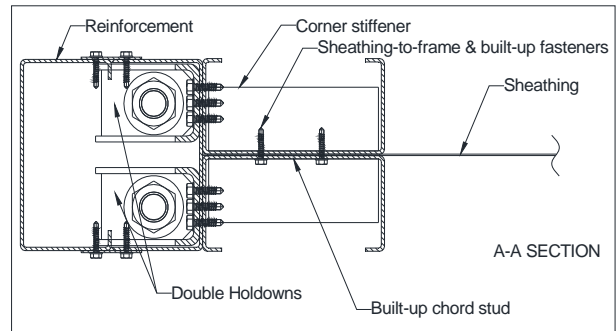
Figure A10: Nominal dimensions and specifications of specimen W25-CR3.
