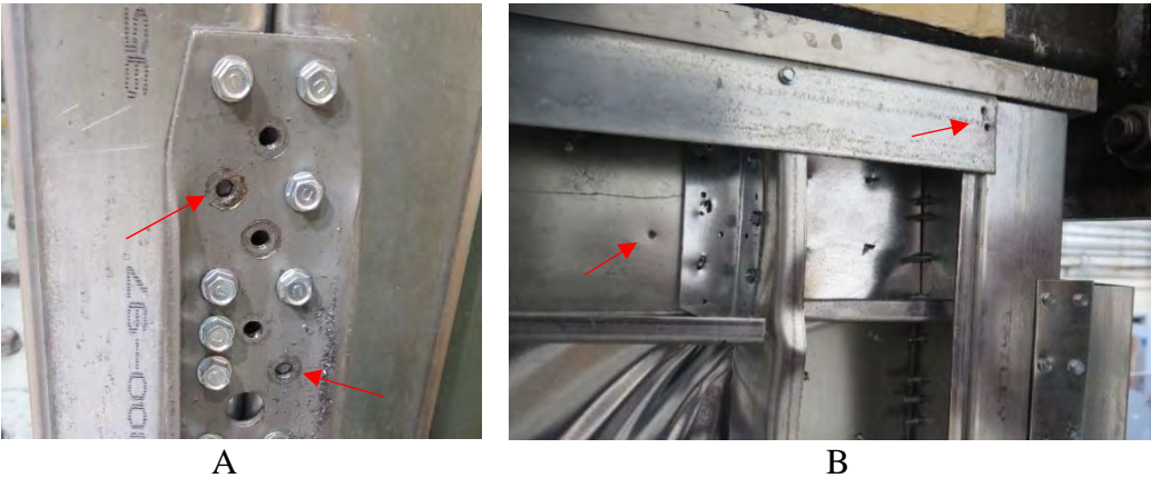
Figure 3.2: A) Shear failure of holddown screws. B) Shear failure of sheathing and track screws.
