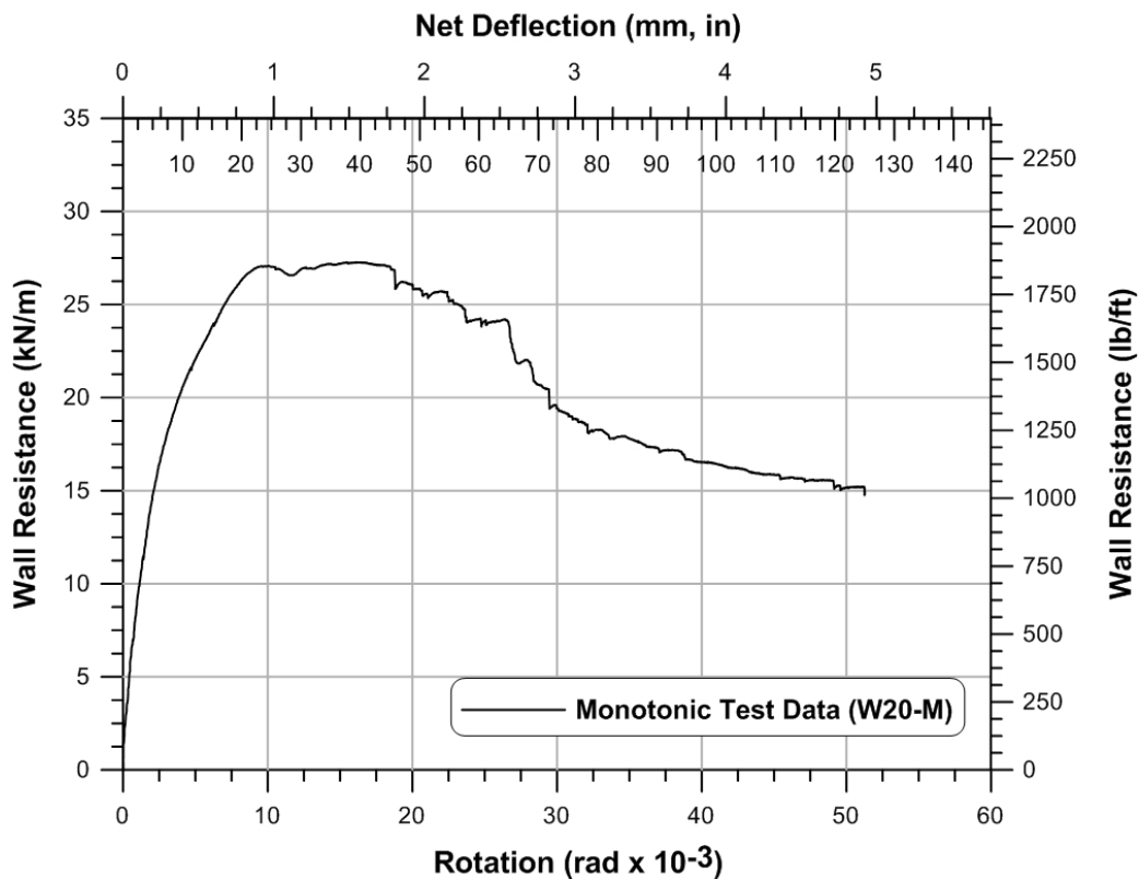
Figure 2.26: Typical monotonic test curve.
