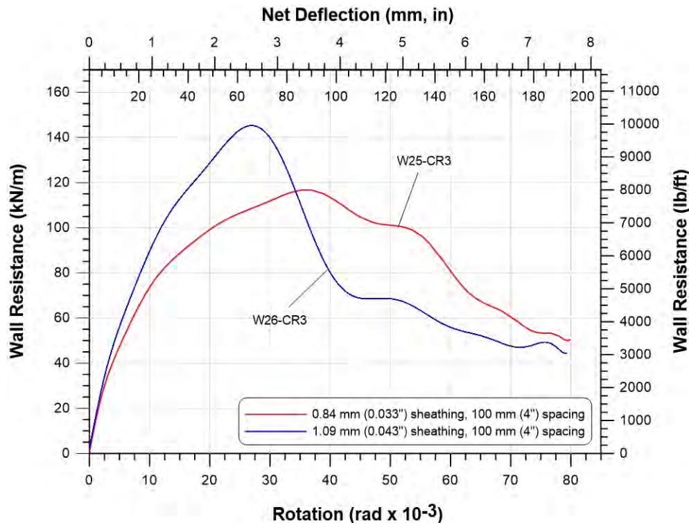
Figure 3.26: Comparison of sheathing thickness between centre-sheathed specimens W25-CR3 and W26-CR3.
