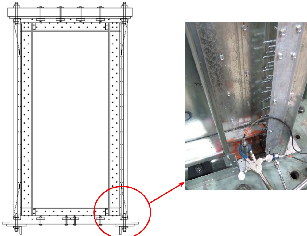
Figure 2.20: MR2 chord stud reinforcement.
