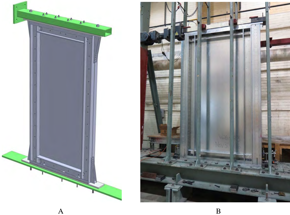
Figure 2.5: Centre-sheathed wall design. A) Original wall configuration. B) Final wall configuration with chord stud reinforcement.
