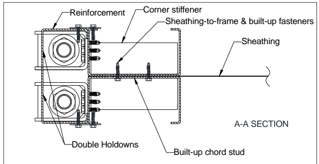
Figure A8: Nominal dimensions and specifications of specimen W16-MR2.
