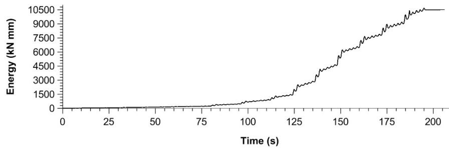
Figure G4: EEEP plot, cyclic test data, and time-history of double-sheathed specimen W20-C.
