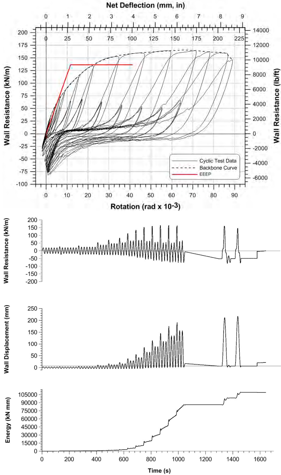
Figure G11: EEEP plot, asymmetric cyclic test data, and time-history of double-sheathed specimen W15B-CR3.
