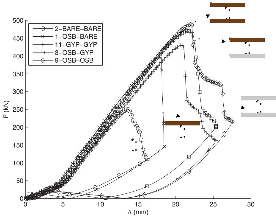
809 Figure 2 – P-Δ curve of full-scale walls comparing different sheathing combinations (note, Δ is 810 overall axial machine displacement, i.e. change in actuator position)
