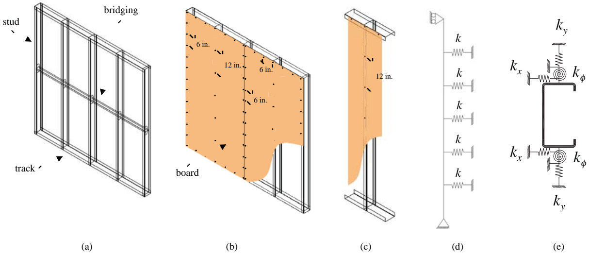
804 Figure 1 – Cold-formed steel walls and bracing of the studs: (a) all steel wall, (b) sheathed wall, 805 (c) sheathed single stud, (d) schematic of stud with springs as bracing at fastener locations, (e) 806 detail of springs bracing the stud cross-section. 807
