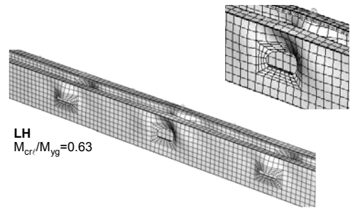
Figure 4.58 Local buckling modes for specimen 6B,18,1&2(H) with and without holes
