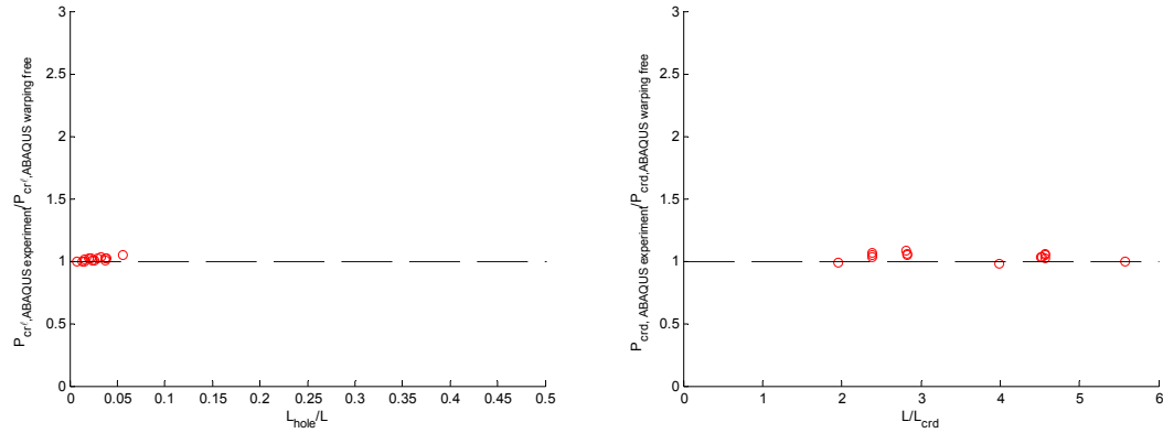
Figure 4.15 Influence of weak-axis pinned boundary conditions versus warping free boundary conditions on (a) P_{cr} as a function of hole length to column length and (b) P_{cr} as a function of column length to member length.
