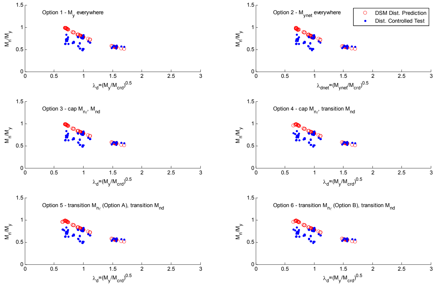
Figure 8.63 Comparison of experimental test strengths to predictions for laterally braced beams with distortional buckling-controlled failures as a function of distortional slenderness
