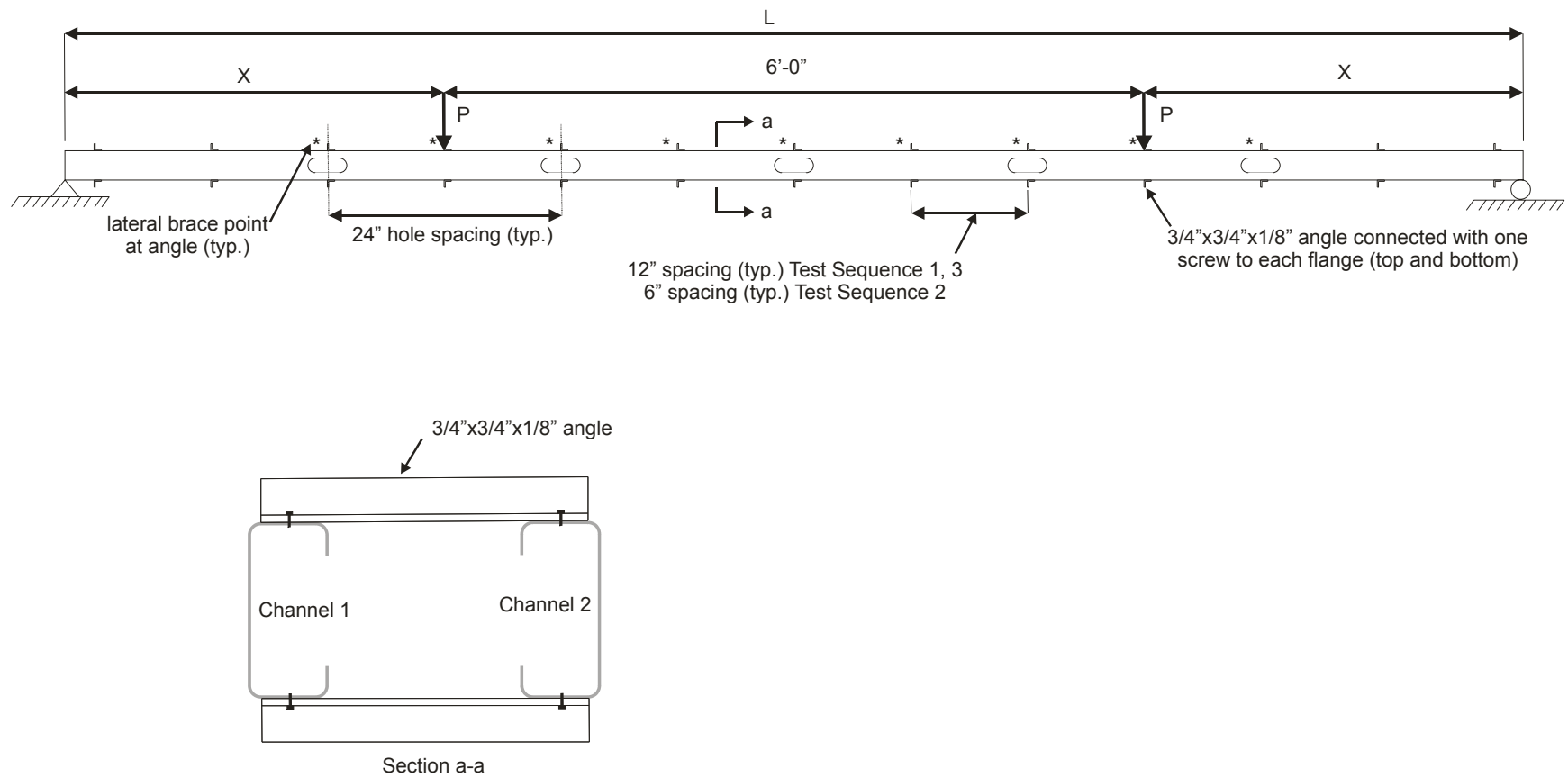
Figure 4.51 Experiment test setup with hole spacing, location of lateral bracing, spacing of aluminum angle straps, and load points
