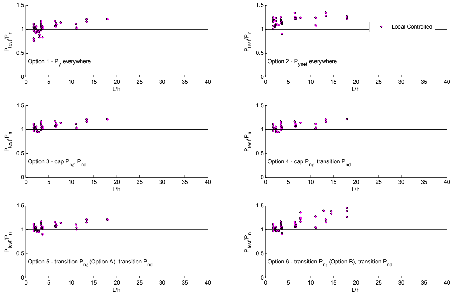
Figure 8.41 Test-to-predicted ratios for experiment local buckling-controlled column failures as a function of column length, L , to flat web width, h
