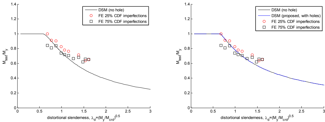
Figure 8.51 Comparison of simulated beam strengths ( I_{net}/I_g=1.0 ) to (a) the existing DSM distortional buckling design curve and to (b) the proposed DSM distortional buckling curve for beams with holes
