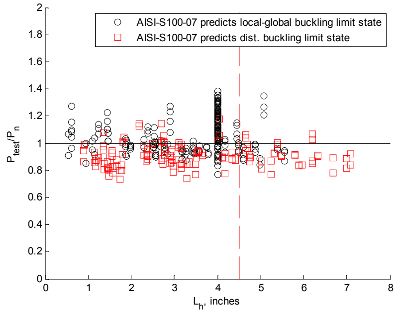
Figure M.4 AISI S100-07 test-to-predicted ratio, FE simulated tests of columns with holes, code requires that hole length L_h \leq 4.5 inches
