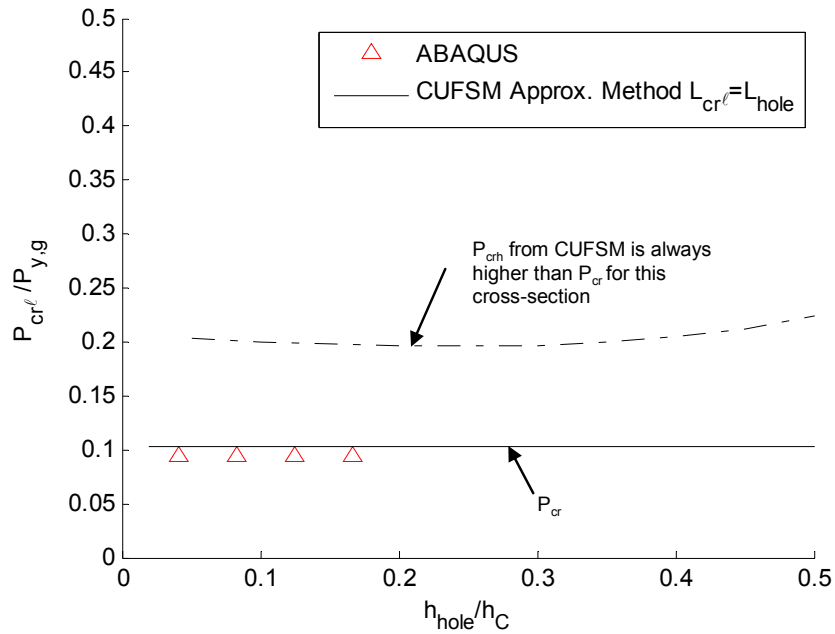
Figure 4.23 ABAQUS results are slightly lower than CUFSM predictions, CUFSM predicts correctly that plate local buckling controls over unstiffened strip buckling.
