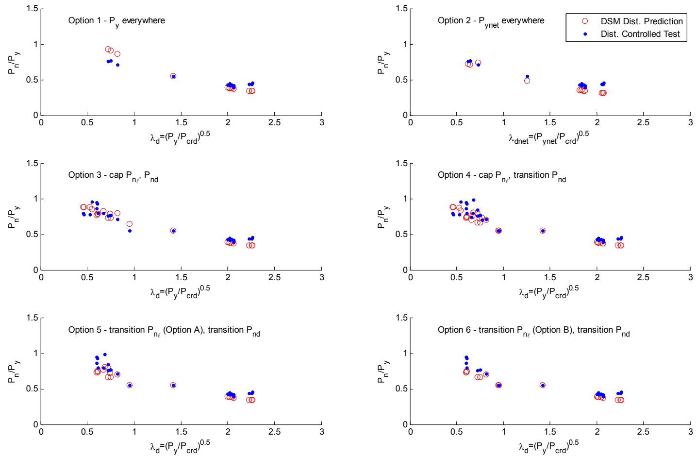
Figure 8.33 Comparison of experimental test strengths to predictions for columns with distortional buckling-controlled failures as a function of distortional slenderness
