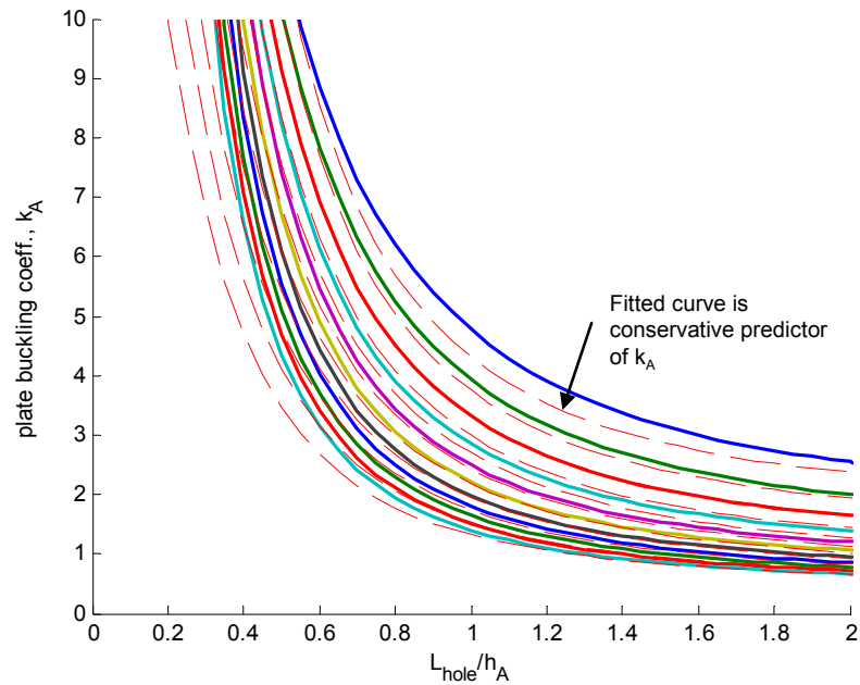
Figure C.3 The fitted curve for k_A is a conservative predictor when L_{hole}/y_A \leq 2
