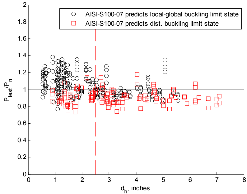
Figure M.3 AISI S100-07 test-to-predicted ratio, FE simulated tests of columns with holes, code requires that hole depth d_h \leq 2.5 inches
