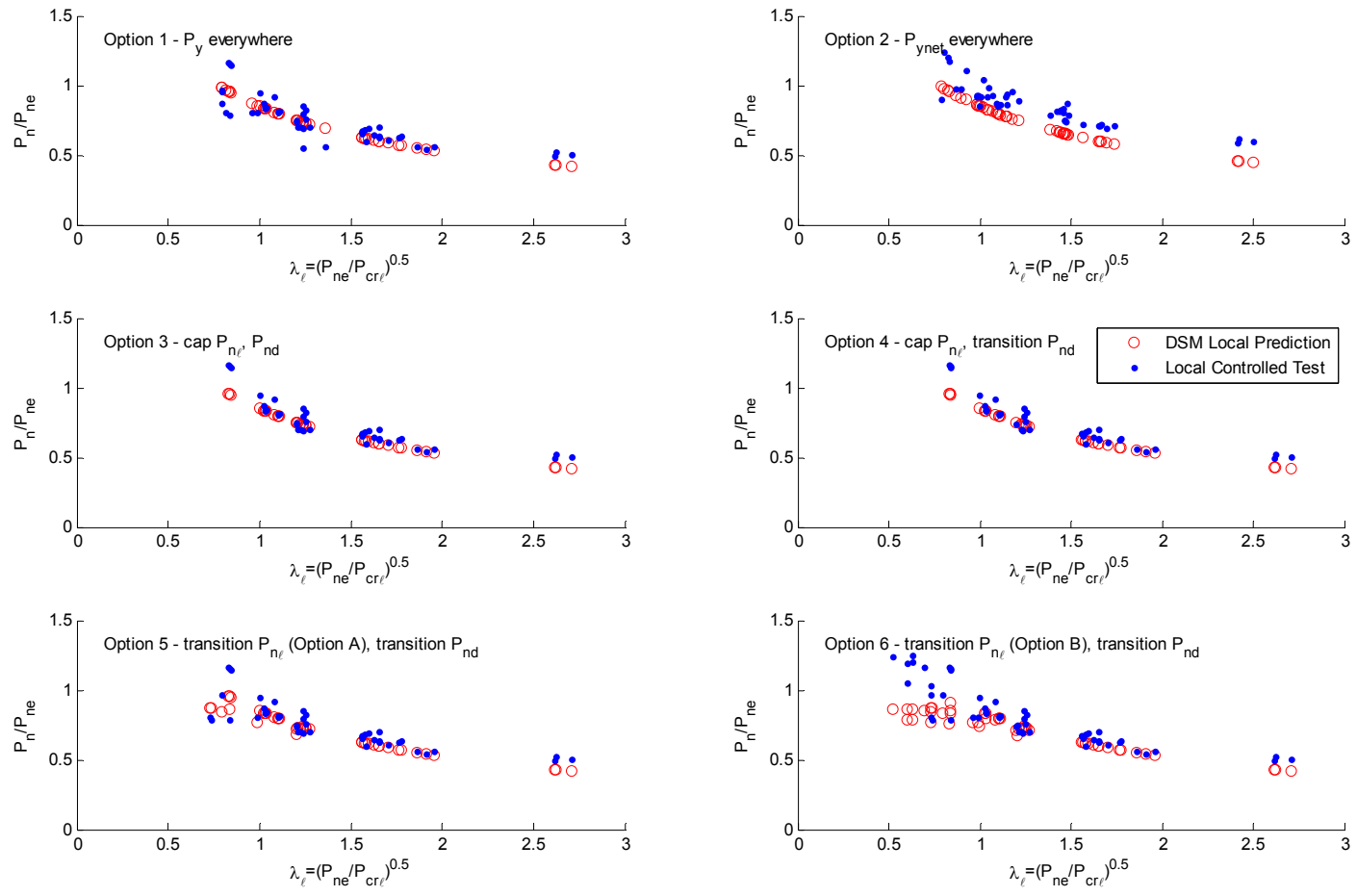
Figure 8.31 Comparison of experimental test strengths to predictions for columns with local buckling-controlled failures as a function of local slenderness (tested strength is normalized by P_{ne} )
