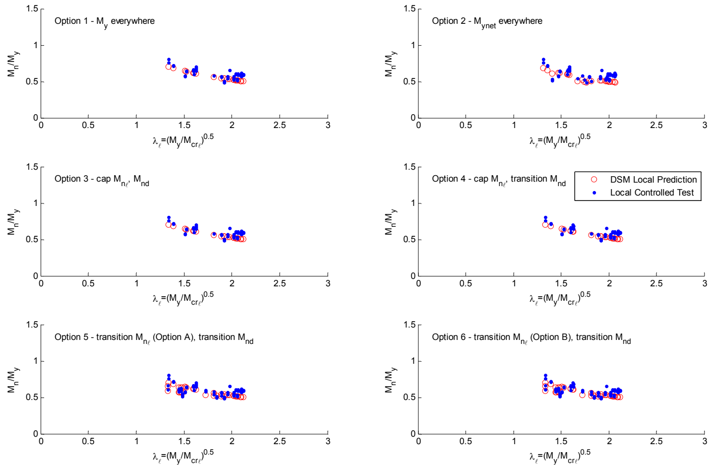
Figure 8.54 Comparison of simulated test strengths to predictions for laterally braced beams with local buckling-controlled failures as a function of local slenderness
