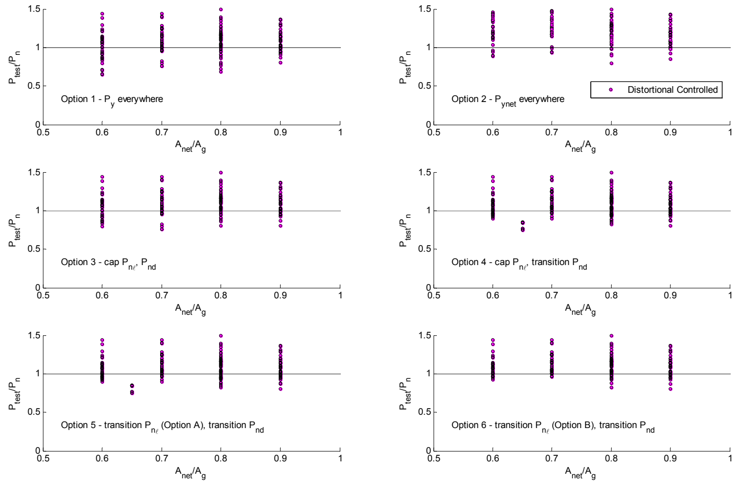
Figure 8.26 Test-to-predicted ratios for simulated distortional buckling-controlled column failures as a function of net cross-sectional area to gross cross-sectional area
