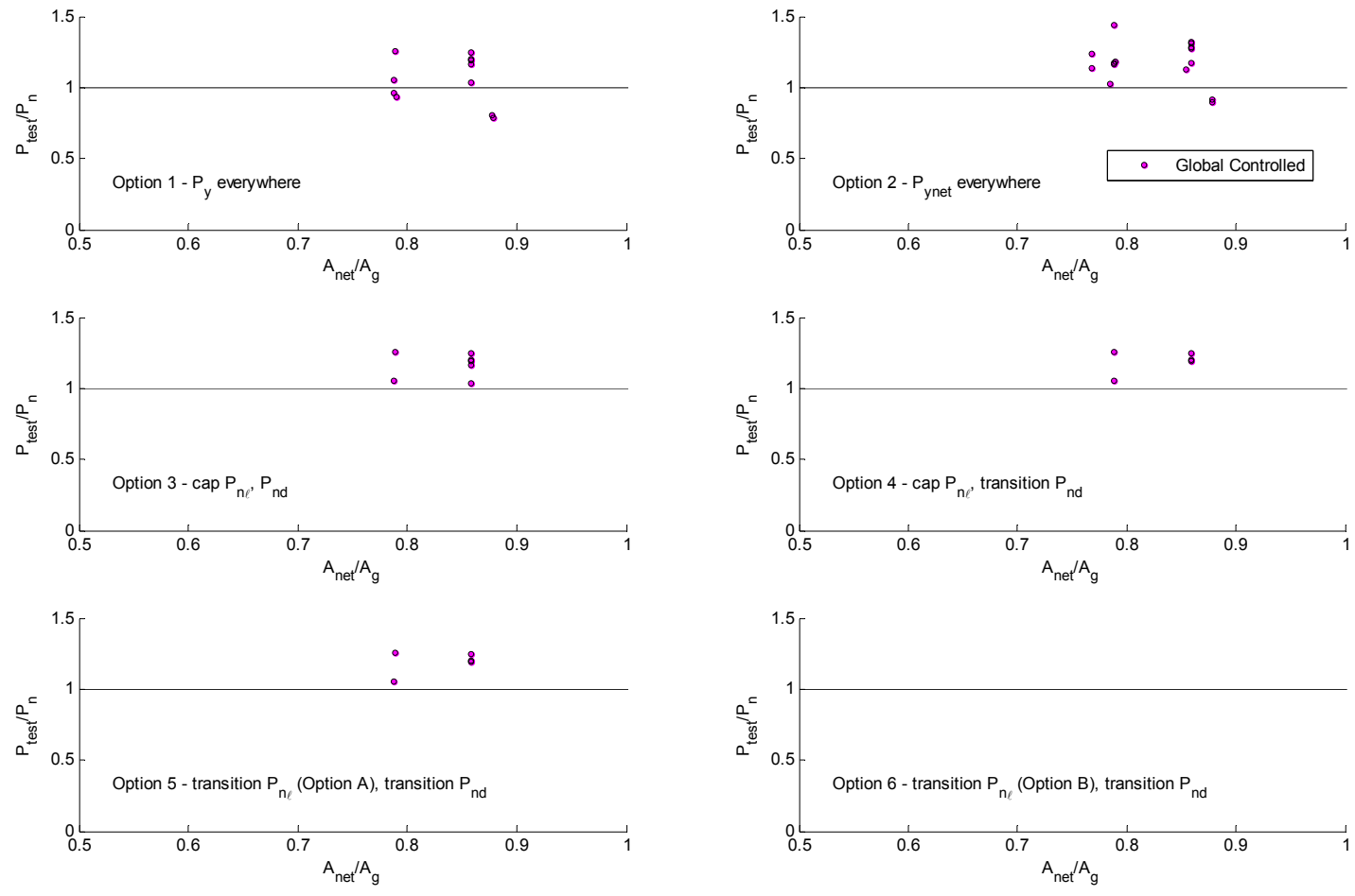
Figure 8.40 Test-to-predicted ratios for experiment global buckling-controlled column failures as a function of net cross-sectional area to gross cross-sectional area
