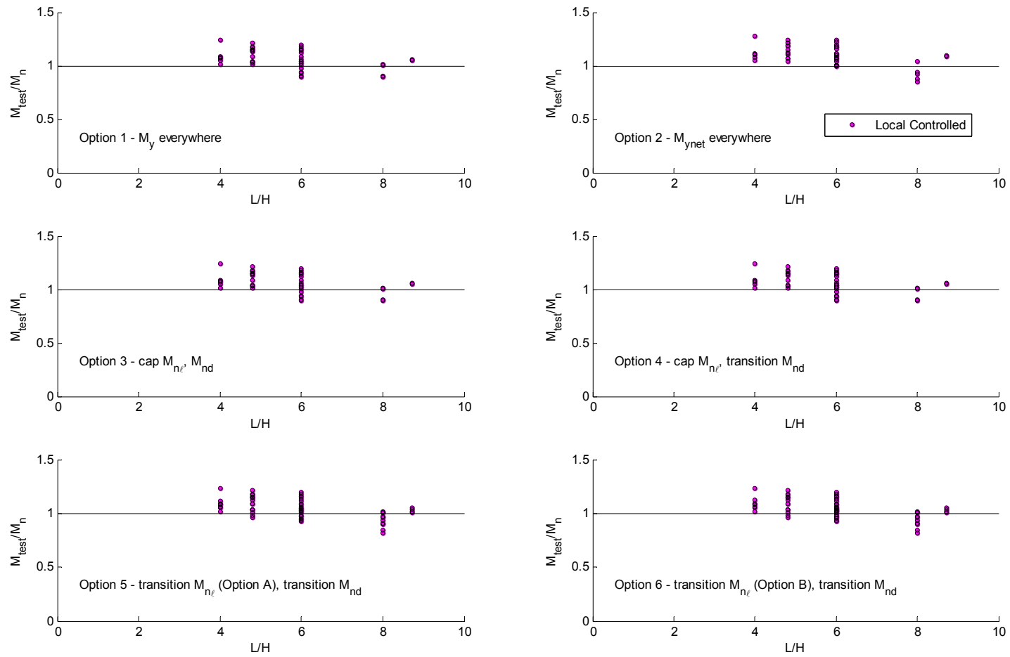
Figure 8.60 Test-to-predicted ratios for simulated local buckling-controlled laterally braced beam failures as a function of column length, L , to beam depth, H
