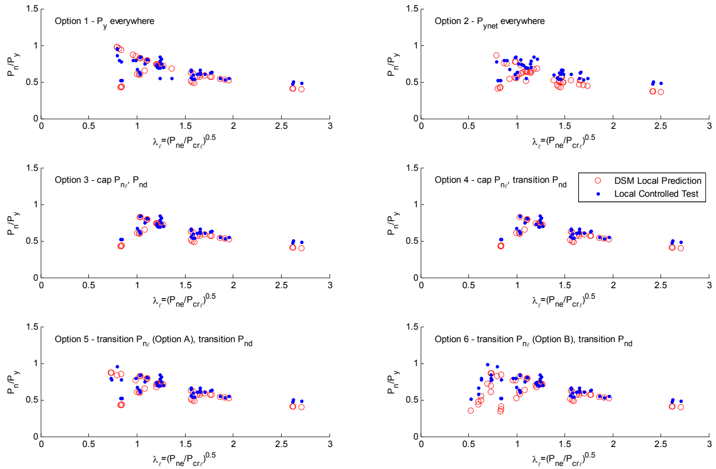
Figure 8.32 Comparison of experimental test strengths to predictions for columns with local buckling-controlled failures as a function of local slenderness (tested strength is normalized by P_y )
