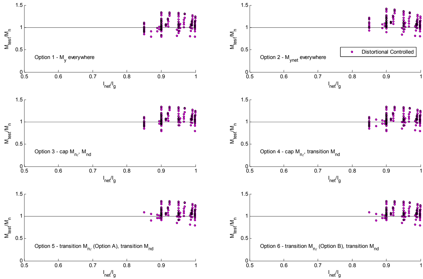
Figure 8.59 Test-to-predicted ratios for simulated distortional buckling-controlled laterally braced beam failures as a function of net cross-sectional moment of inertia to gross cross-sectional moment of inertia
