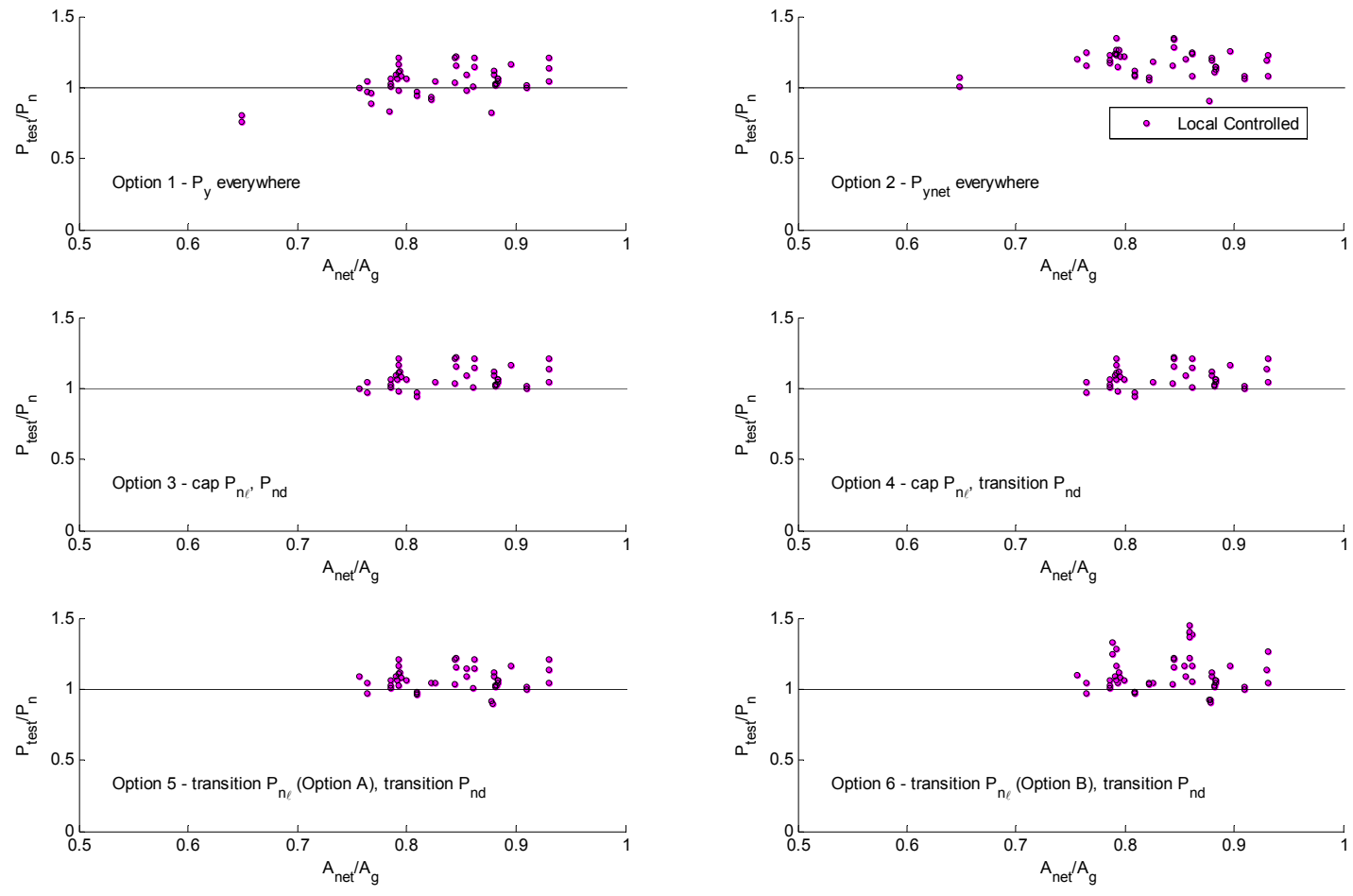
Figure 8.38 Test-to-predicted ratios for experiment local buckling-controlled column failures as a function of net cross-sectional area to gross cross-sectional area
