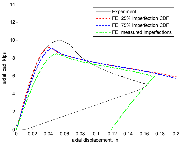
Figure 7.41 Load-displacement response of specimen 362-1-24-H
