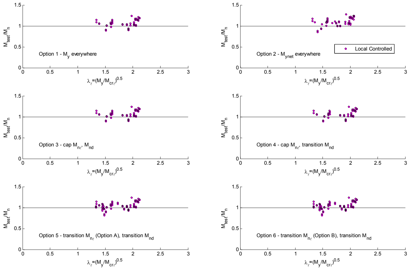
Figure 8.56 Test-to-predicted ratios for local buckling-controlled simulated laterally braced beam failures as a function of local slenderness
