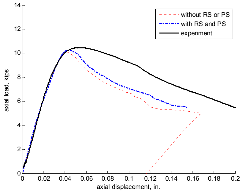
Figure 7.49 Influence of residual stresses (RS) and plastic strains (PS) on the FE load-displacement response of specimen 362-1-24-NH.
