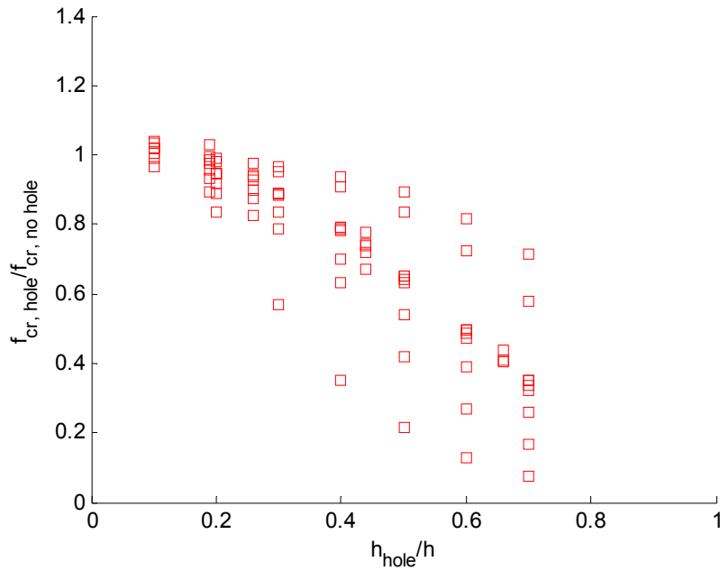
Figure 3.40 The presence of holes causes a decrease in critical elastic buckling load for unstiffened plates in uniaxial compression.
