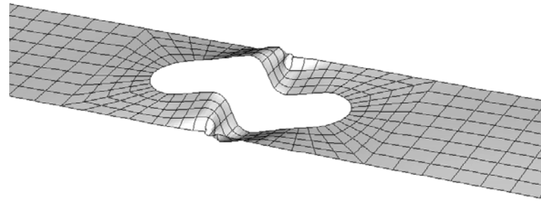
Figure 7.10 Deformation at ultimate load of a stiffened element with a hole loaded in compression. The common failure mechanism is material yielding adjacent to the hole followed by plate folding.
