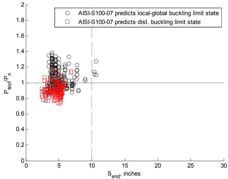
Figure M.6 AISI S100-07 test-to-predicted ratio, FE simulated tests of columns with holes, code requires clear hole spacing at column ends S_{end} \geq 10 inches
