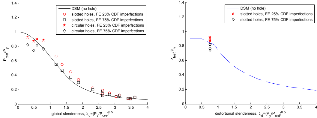
Figure 8.10 Comparison of simulated column strengths ( A_{net}/A_g=0.90 ) to (a) the existing DSM global buckling design curve and to (b) the proposed DSM distortional buckling curve for columns with holes
