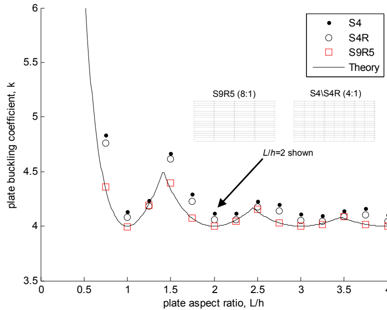
Figure 2.3 Accuracy of ABAQUS S9R5, S4, and S4R elements for a stiffened element with varying aspect ratios, 8:1 finite element aspect ratio for the S9R5 element, 4:1 element aspect ratio for the S4 and S4R elements
