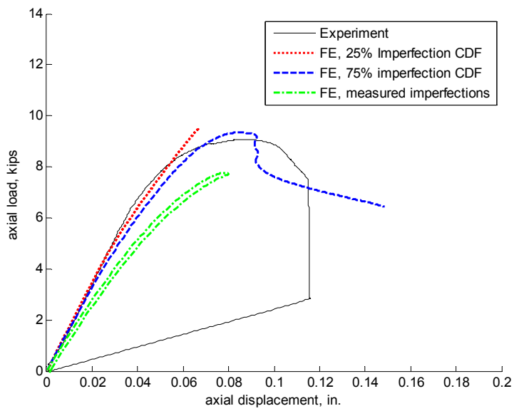
Figure 7.42 Load-displacement response of specimen 362-1-48-NH
