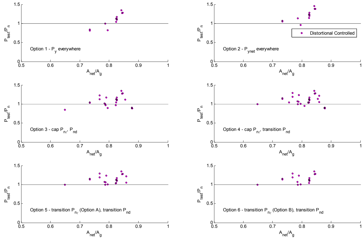
Figure 8.39 Test-to-predicted ratios for experiment distortional buckling-controlled column failures as a function of net cross-sectional area to gross cross-sectional area
