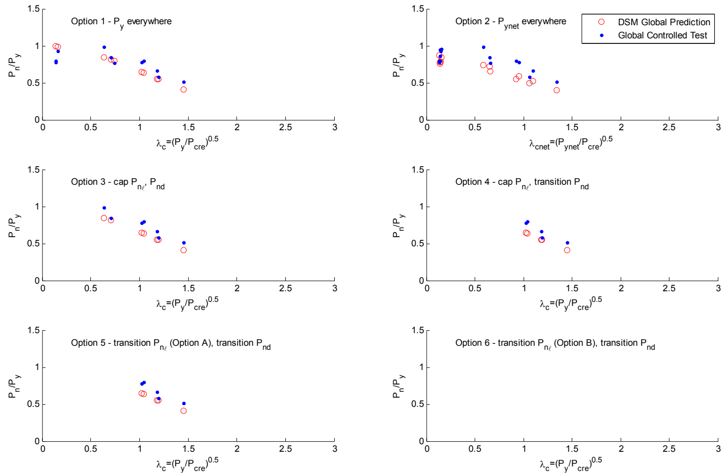
Figure 8.34 Comparison of experimental test strengths to predictions for columns with global buckling-controlled failures as a function of global slenderness
