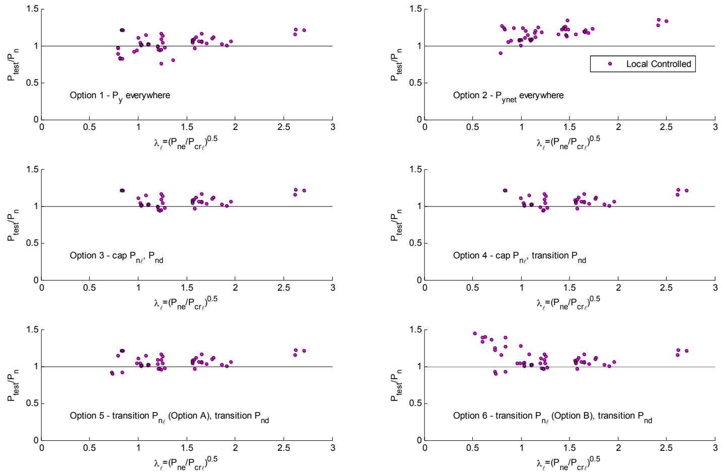
Figure 8.35 Test-to-predicted ratios for experiment local buckling-controlled column failures as a function of local slenderness
