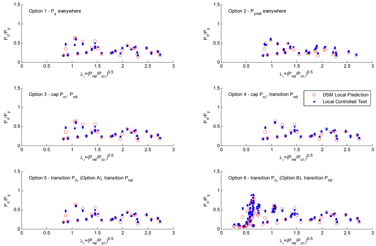
Figure 8.19 Comparison of simulated test strengths to predictions for columns with local buckling-controlled failures as a function of local slenderness (tested strength is normalized by P_{yg} )
