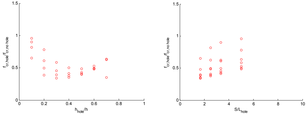
Figure 3.26 Influence of slotted holes on critical elastic buckling stress f_{cr} of stiffened elements in bending as a function of (a) hole size relative to plate width and (b) hole spacing as a function of hole length.
