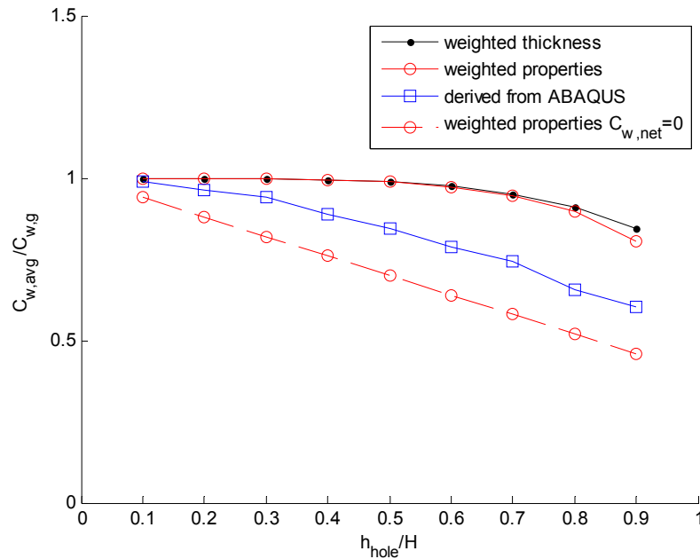
Figure 4.46 Comparison of “weighted thickness” and “weighted properties” approximations to the ABAQUS derived warping torsion constant C_{w,avg} .
