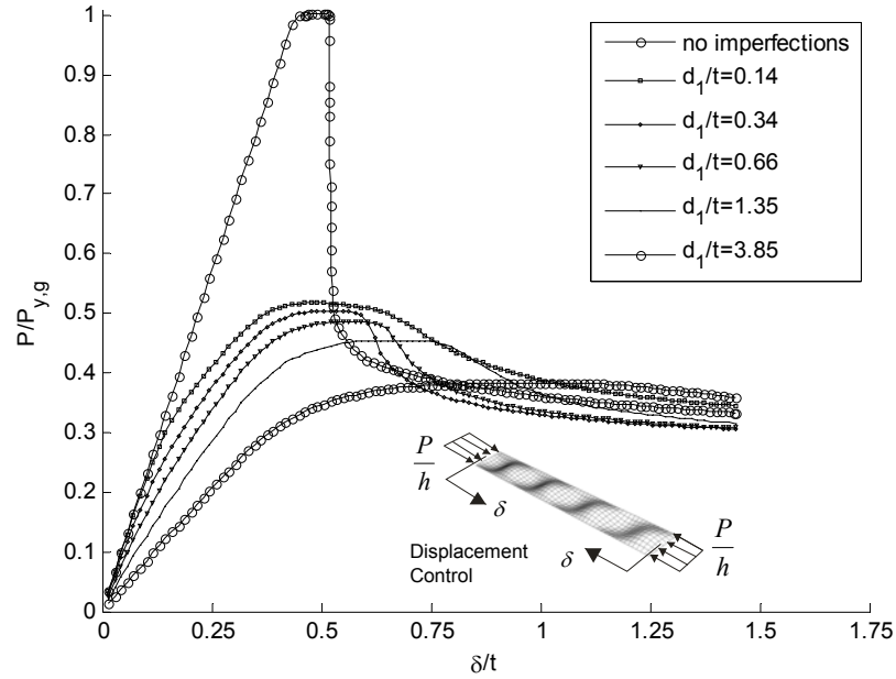
Figure 7.17 Load-displacement sensitivity to imperfection magnitude for a plate without a hole
