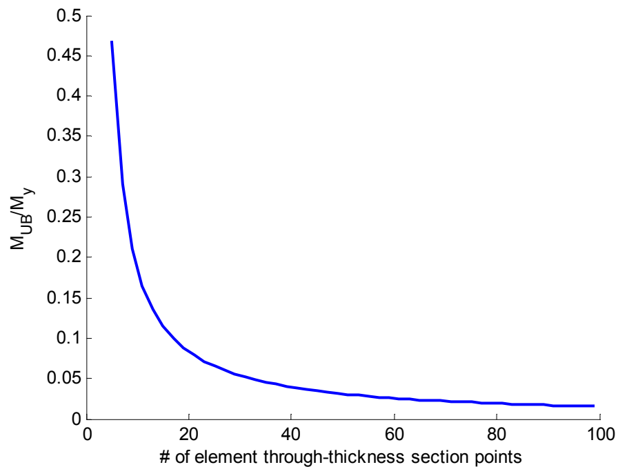
Figure 7.39 Influence of section points on the unbalanced moment (accuracy) of the transverse residual stress distribution as implemented in ABAQUS
