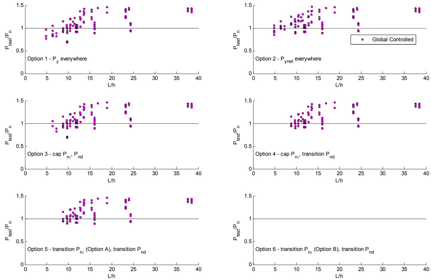
Figure 8.30 Test-to-predicted ratios for simulated global buckling-controlled column failures as a function of column length, L , to web width, h
