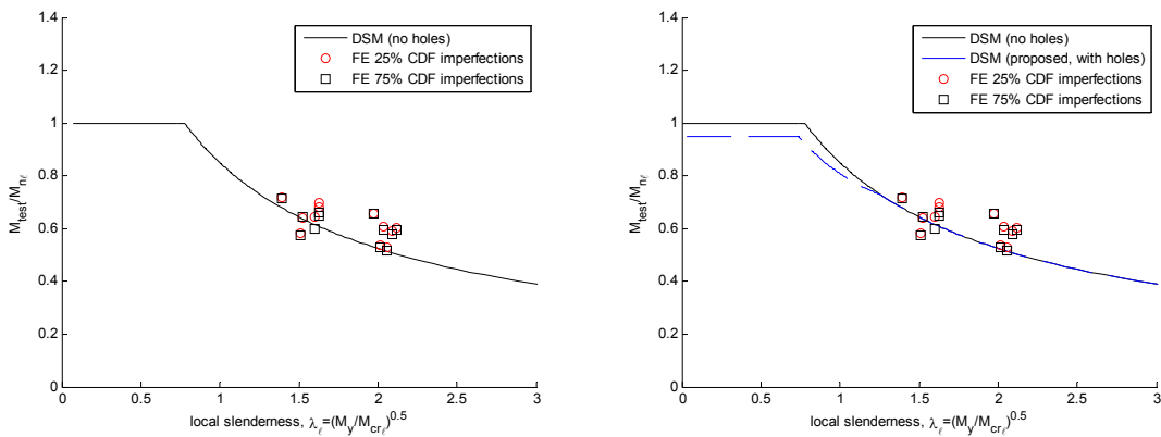
Figure 8.47 Comparison of simulated beam strengths ( I_{net}/I_g=0.95 ) to (a) the existing DSM local buckling design curve and to (b) the proposed DSM local buckling curve for beams with holes
