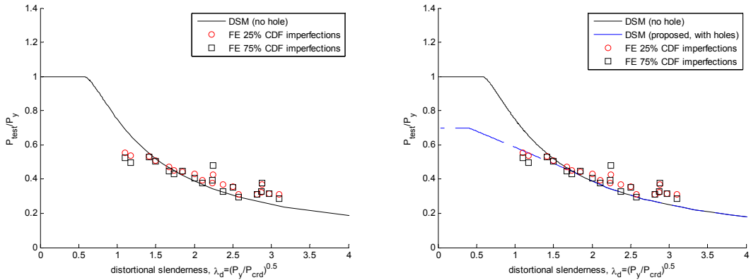
Figure 8.6 Comparison of simulated column strengths ( A_{net}/A_g=0.80 ) to (a) the existing DSM distortional buckling design curve and to (b) the proposed DSM distortional buckling curve for columns with holes
