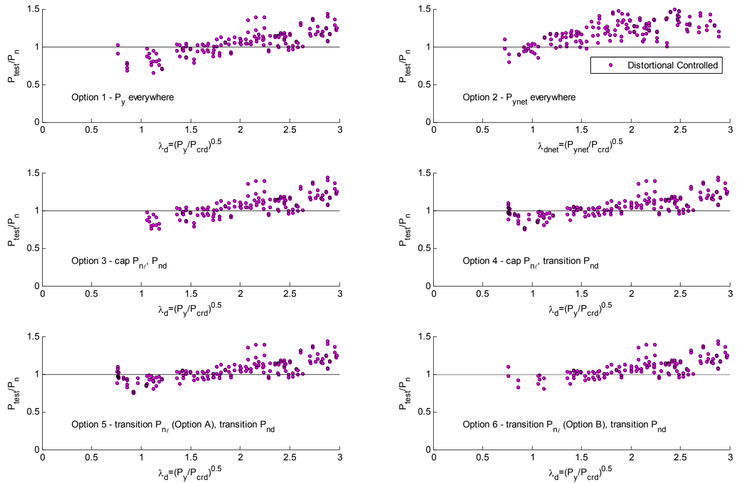
Figure 8.23 Test-to-predicted ratios for distortional buckling-controlled simulated column failures as a function of distortional slenderness
