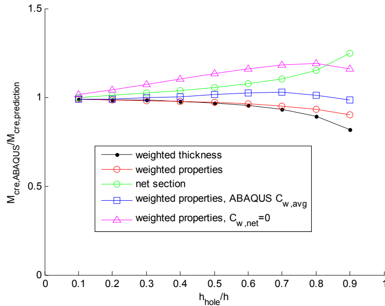
Figure 4.78 Comparison of “weighted thickness” and “weighted properties” prediction methods for the SSMA 1200S162-68 lateral-torsional beam buckling mode. Predictions using net section properties are also plotted as a conservative benchmark.
