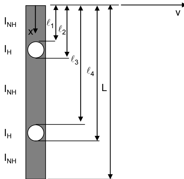
Figure E.1 Long column with two holes spaced symmetrically about the longitudinal midline.
