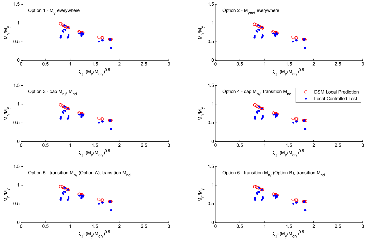
Figure 8.62 Comparison of experimental test strengths to predictions for laterally braced beams with local buckling-controlled failures as a function of local slenderness
