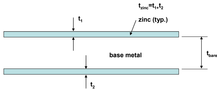
Figure 5.16 Base metal and zinc thickness definitions
