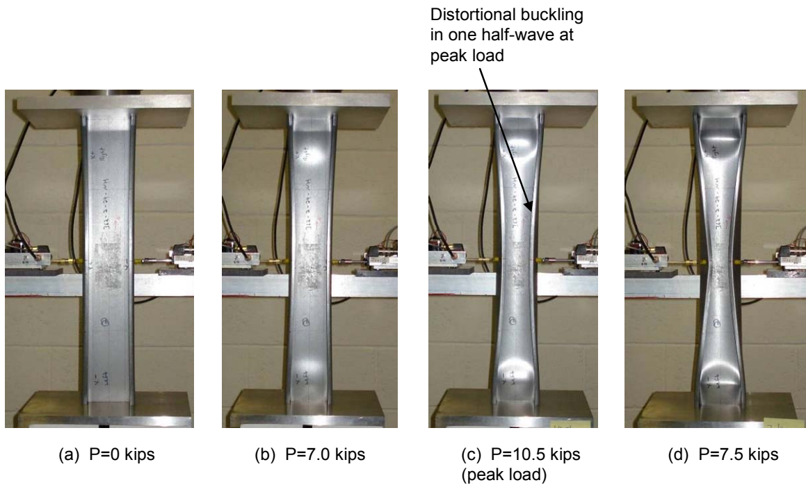
Figure 5.36 Load-displacement progression for short column specimen 362-2-24-NH
