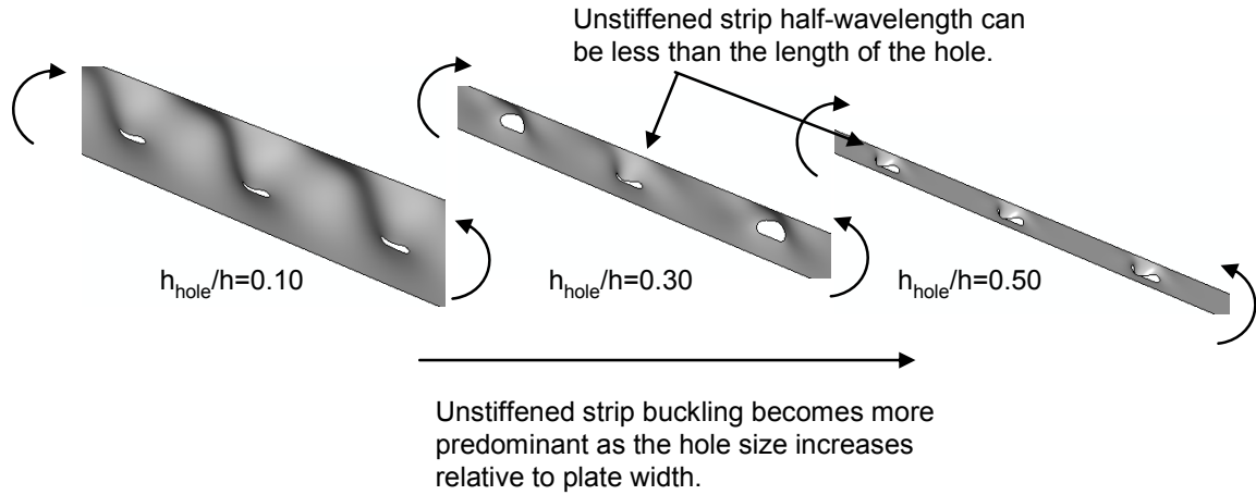
Figure 3.25 Stiffened plates loaded with a linear bending stress gradient exhibit buckling of the unstiffened strip adjacent to the hole in the compression region of the plate.
