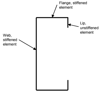
Figure 3.1 Stiffened and unstiffened elements in a lipped C-section
