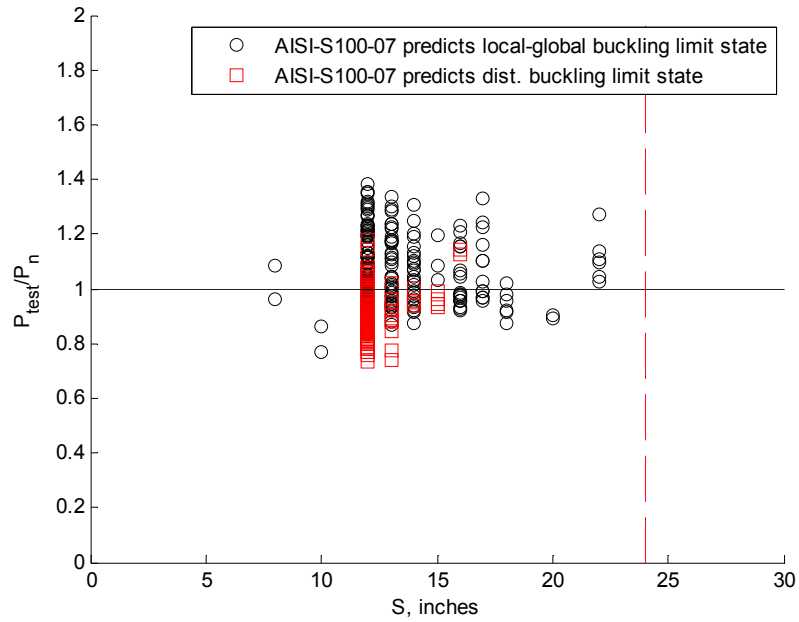
Figure M.5 AISI S100-07 test-to-predicted ratio, FE simulated tests of columns with holes, code requires hole spacing S \geq 24 inches
