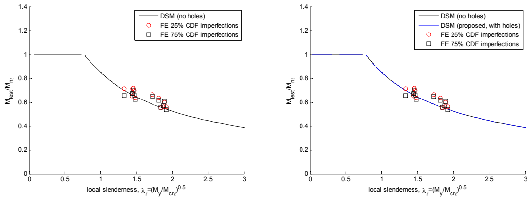
Figure 8.46 Comparison of simulated beam strengths ( I_{net}/I_g=1.0 , no holes) to (a) the existing DSM local buckling design curve and to (b) the proposed DSM local buckling curve for beams with holes
