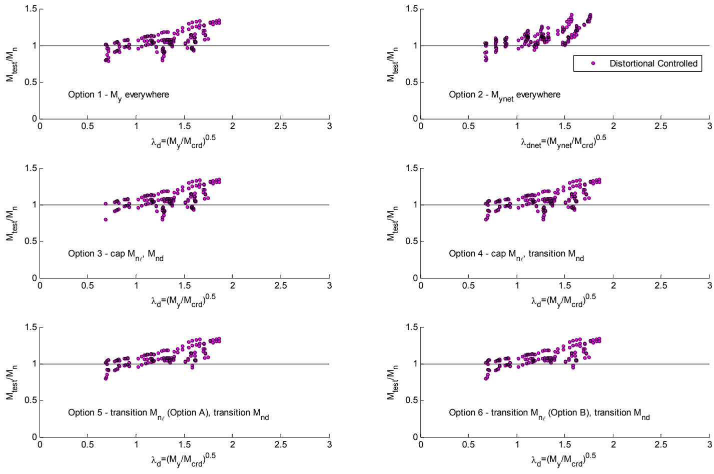
Figure 8.57 Test-to-predicted ratios for distortional buckling-controlled simulated laterally braced beam failures as a function of distortional slenderness
