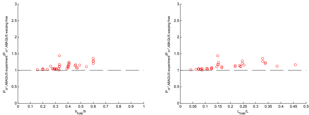
Figure 4.14 Influence of fixed-fixed boundary conditions versus warping free boundary conditions on P_{cr\ell} for column experiments ( L/H < 4 ) as a function of (a) hole width relative to column width and (b) hole length relative to column length
