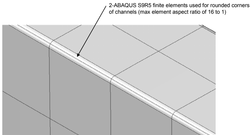
Figure 4.54 ABAQUS meshing details for C-section rounded corners
