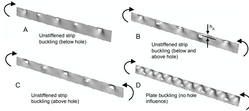
Figure 3.28 The buckled mode shape changes as slotted holes move from the compression region to the tension region of a stiffened element in bending ( h_{hole}/h=0.20 ).
