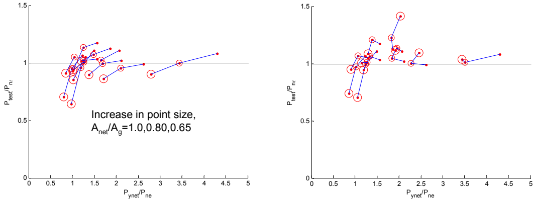
Figure 8.14 Comparison of column test-to-prediction ratios for columns failing by local-global buckling interaction as a function of P_{yne}/P_{ne} where P_{ne} is calculated (a) without the influence of holes (b) and with the influence of holes
