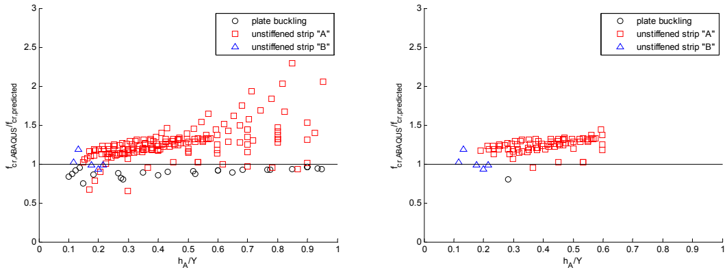
Figure 3.35 Influence of h_A/Y on the accuracy of the prediction method for stiffened elements in bending (a) without and (b) with the dimensional limits defined in Eq. (3.9), Eq. (3.24), Eq. (3.25), and Eq. (3.26).
