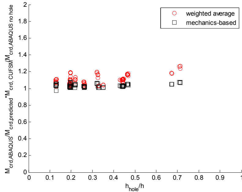
Figure 4.76 Comparison of “mechanics-based” and “weighted-average” prediction methods to ABAQUS results for the distortional buckling load M_{\text{crd}} of C-sections with holes in the elastic buckling database
