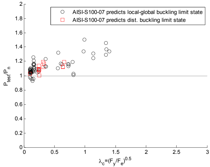
Figure M.1 AISI S100-07 test-to-predicted ratio for experiments on columns with holes, predictions become increasingly conservative with increasing global slenderness
