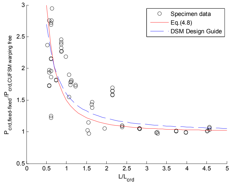
Figure 4.33 Warping-fixed boundary condition amplification of P_{cr,d}
