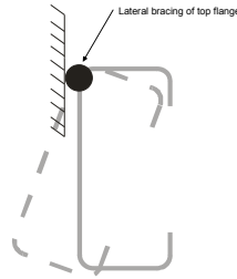
Figure 4.67 Possible global buckling mode occurs about the compression flange lateral brace point
