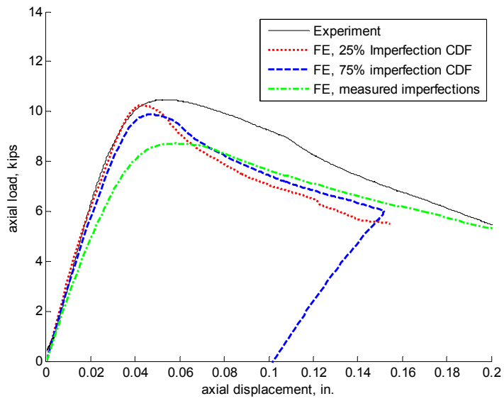
Figure 7.40 Load-displacement response of specimen 362-1-24-NH
