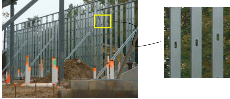
Figure 1.1 Perforations are provided in structural studs to accommodate utilities in the walls of buildings
