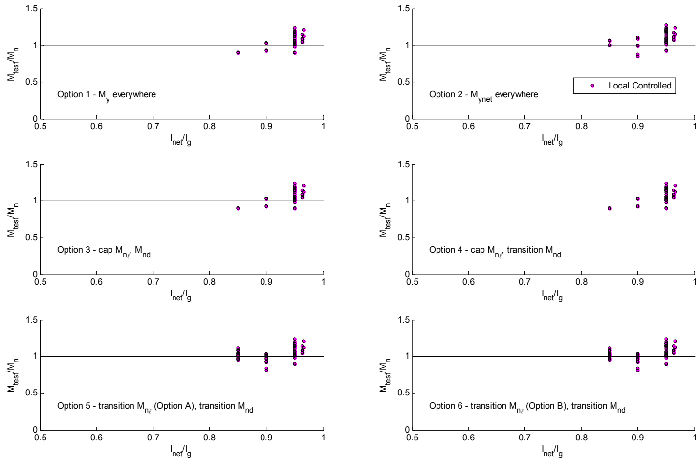
Figure 8.58 Test-to-predicted ratios for simulated local buckling-controlled laterally braced beam failures as a function of net cross-sectional moment of inertia to gross cross-sectional moment of inertia
