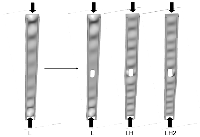
Figure 4.5 The presence of a hole creates unique local buckling modes where unstiffened strip buckling adjacent to the hole occurs symmetrically (LH) or asymmetrically (LH2) increase the distortional tendency of the flanges
