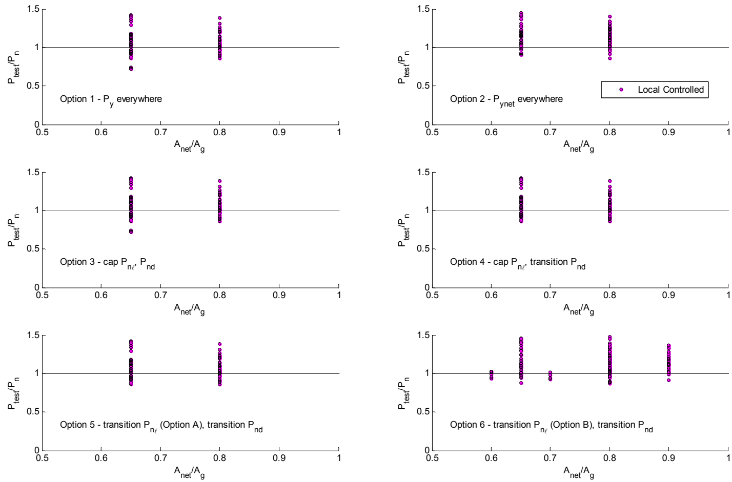
Figure 8.25 Test-to-predicted ratios for simulated local buckling-controlled column failures as a function of net cross-sectional area to gross cross-sectional area
