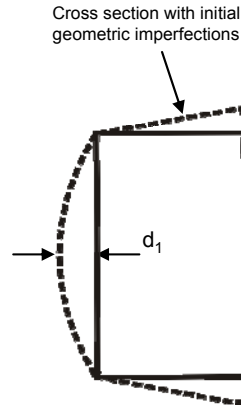
Figure 7.4 Type 1 imperfection (Schafer and Peköz 1998)
