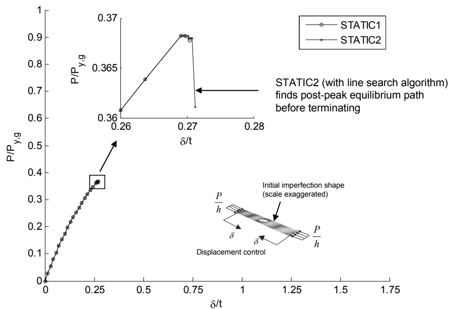
Figure 7.13 STATIC1 and STATIC2 load-displacement curves demonstrate convergence difficulties near the peak load.
