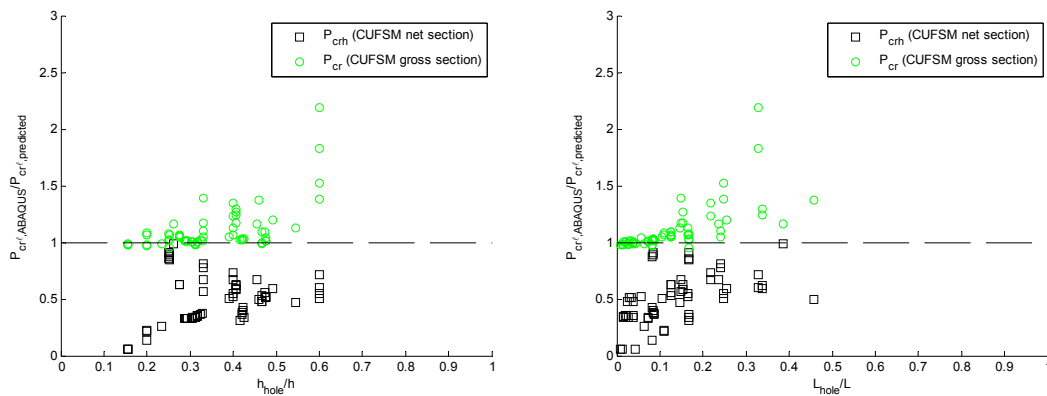
Figure 4.24 Predicted P_{crh} (CUFSM, buckling of the net cross-section) and P_{cr} (CUFSM, buckling of the gross cross section, no hole) are compared relative to the ABAQUS P_{cr\ell} with experiment boundary conditions as a function of (a) hole width to flat web width and (b) hole length to column length
