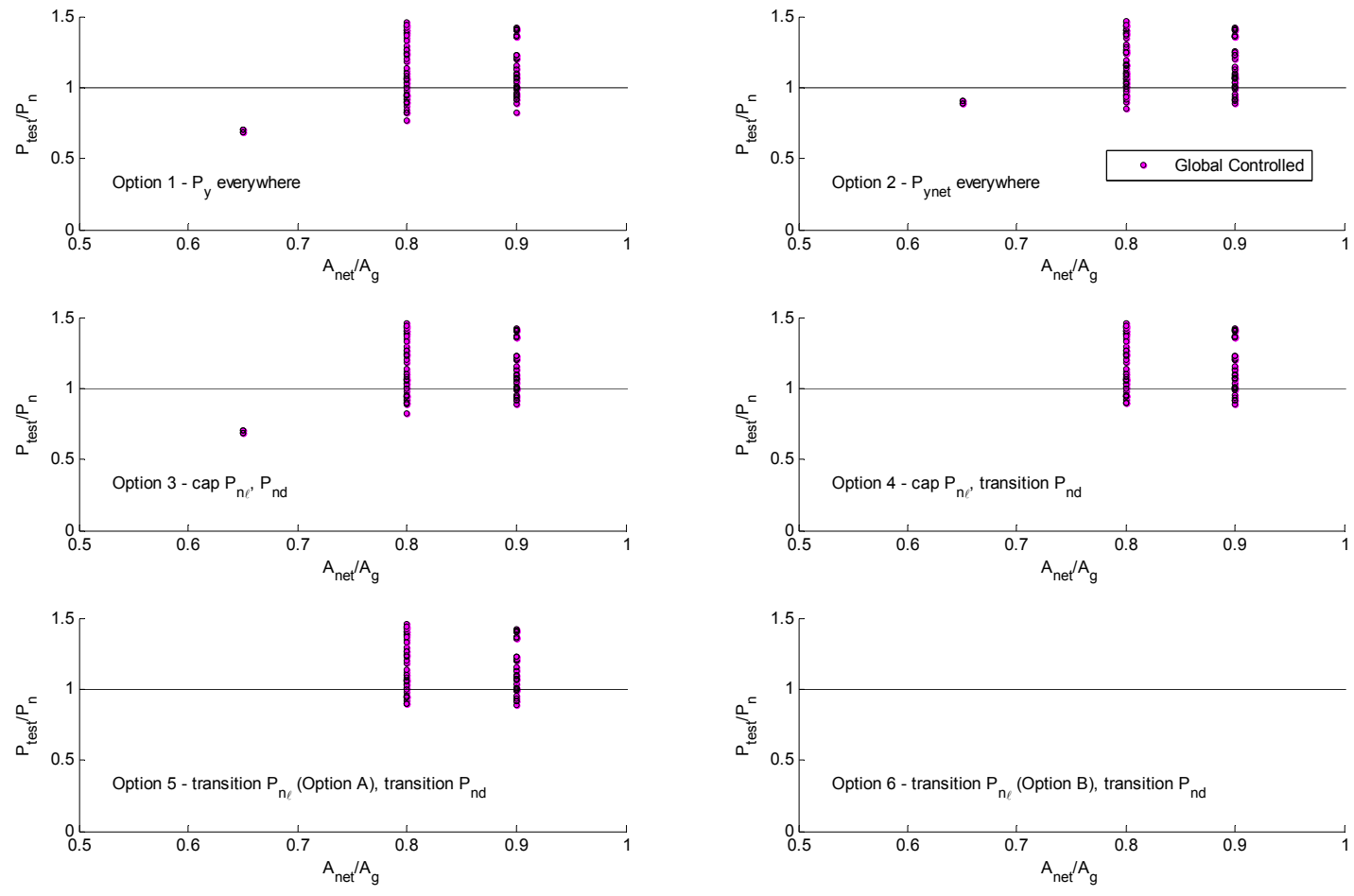
Figure 8.27 Test-to-predicted ratios for simulated global buckling-controlled column failures as a function of net cross-sectional area to gross cross-sectional area
