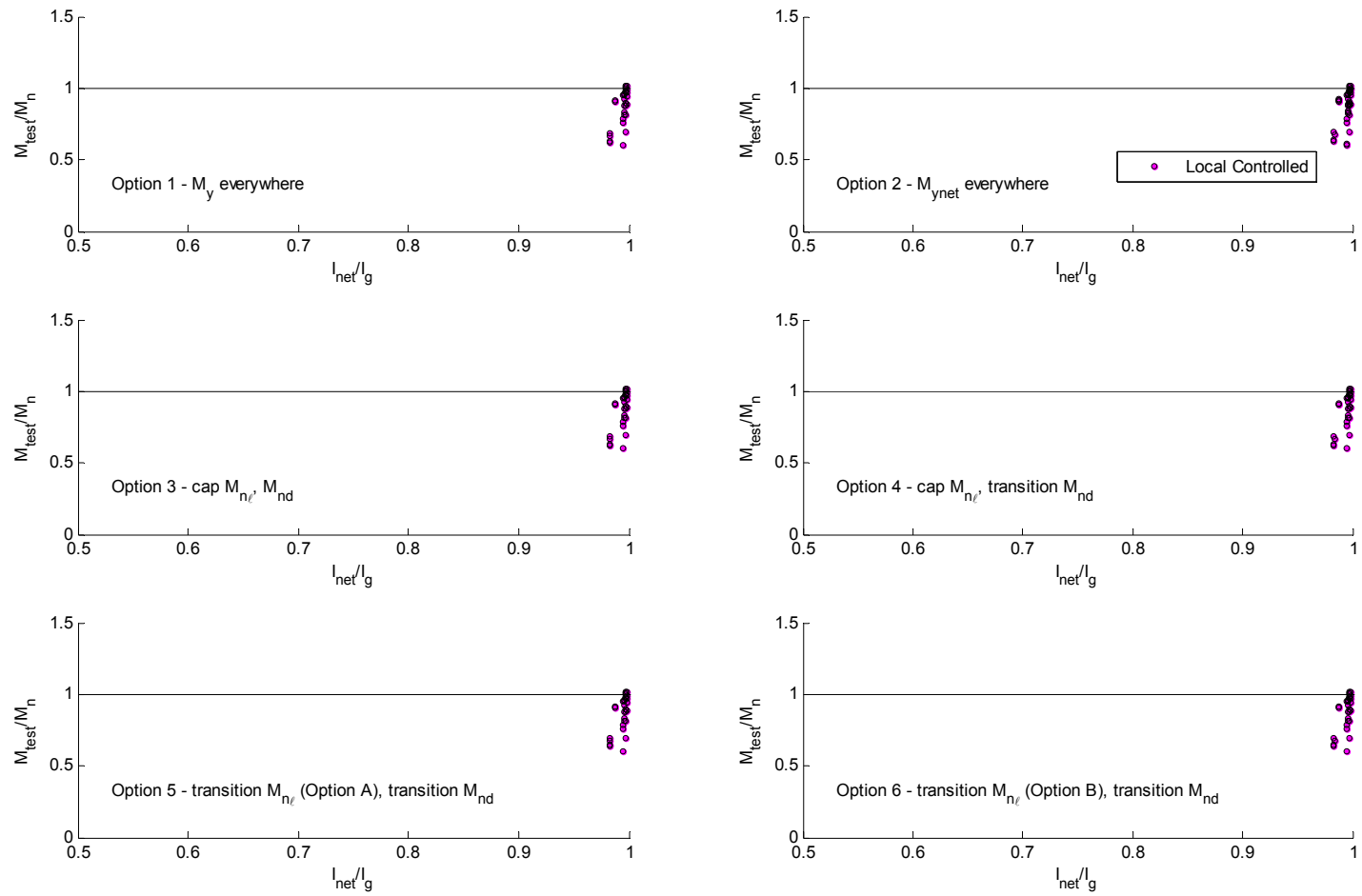
Figure 8.64 Test-to-predicted ratios for experimental local buckling-controlled laterally braced beam failures as a function of net cross-sectional moment of inertia to gross cross-sectional moment of inertia
