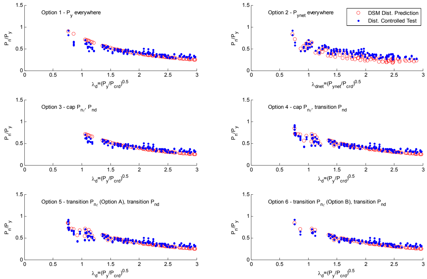
Figure 8.20 Comparison of simulated test strengths to predictions for columns with distortional buckling-controlled failures as a function of distortional slenderness
