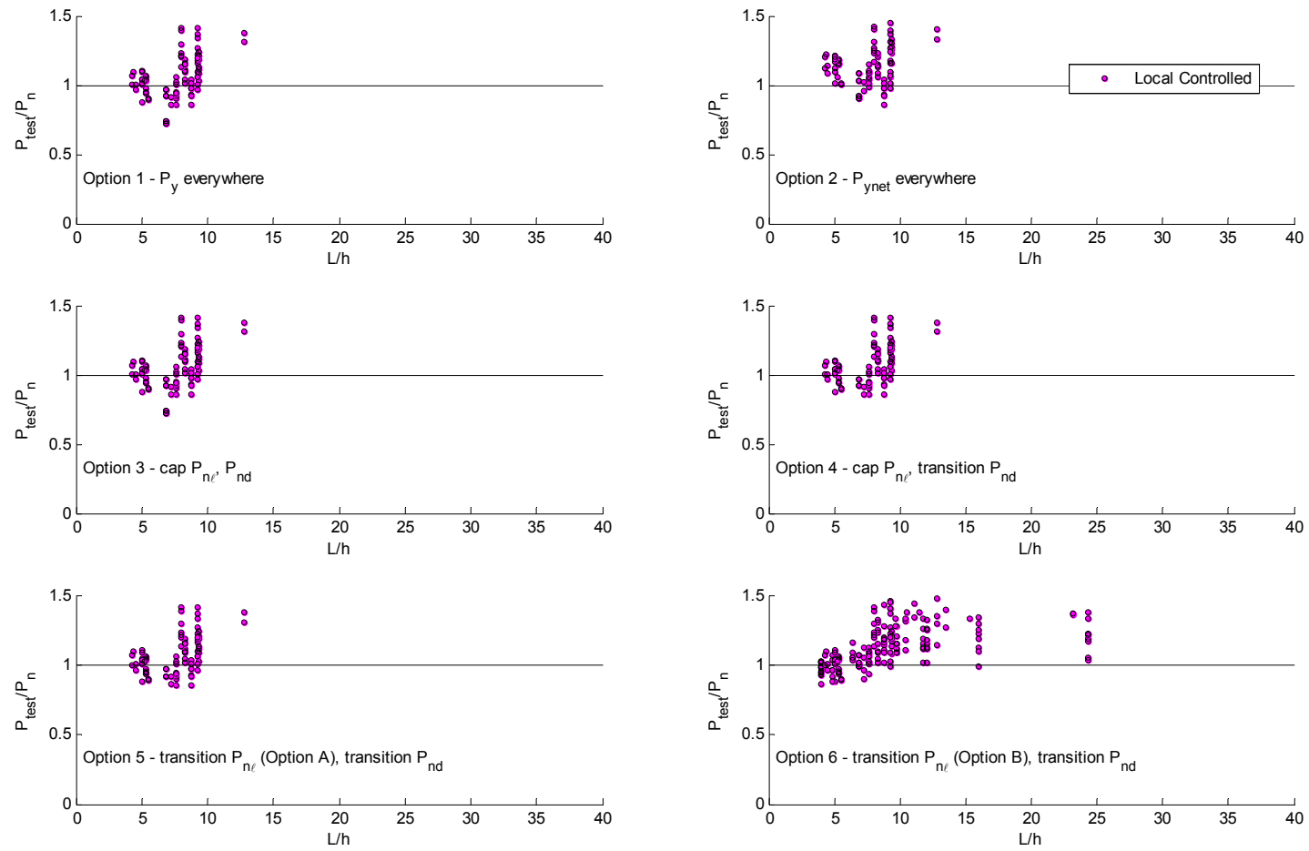
Figure 8.28 Test-to-predicted ratios for simulated local buckling-controlled column failures as a function of column length, L , to flat web width, h
