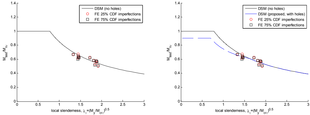
Figure 8.48 Comparison of simulated beam strengths ( I_{net}/I_g=0.90 ) to (a) the existing DSM local buckling design curve and to (b) the proposed DSM local buckling curve for beams with holes
