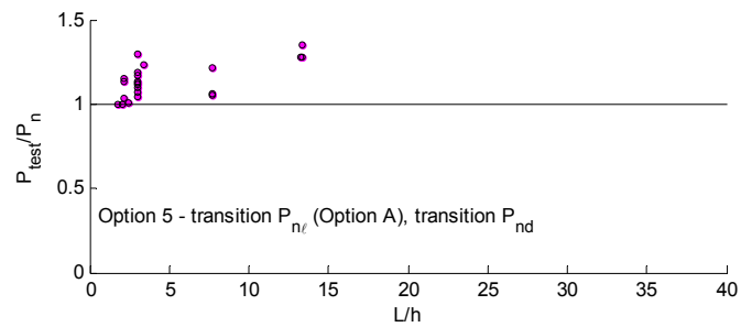
Figure 8.42 Test-to-predicted ratios for experiment distortional buckling-controlled column failures as a function of column length, L , to flat web width, h
