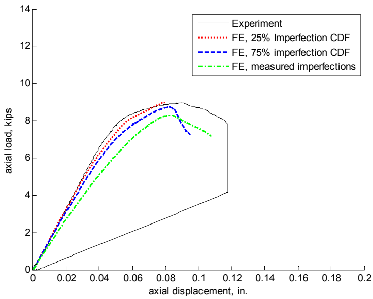
Figure 7.43 Load-displacement response of specimen 362-1-48-H
