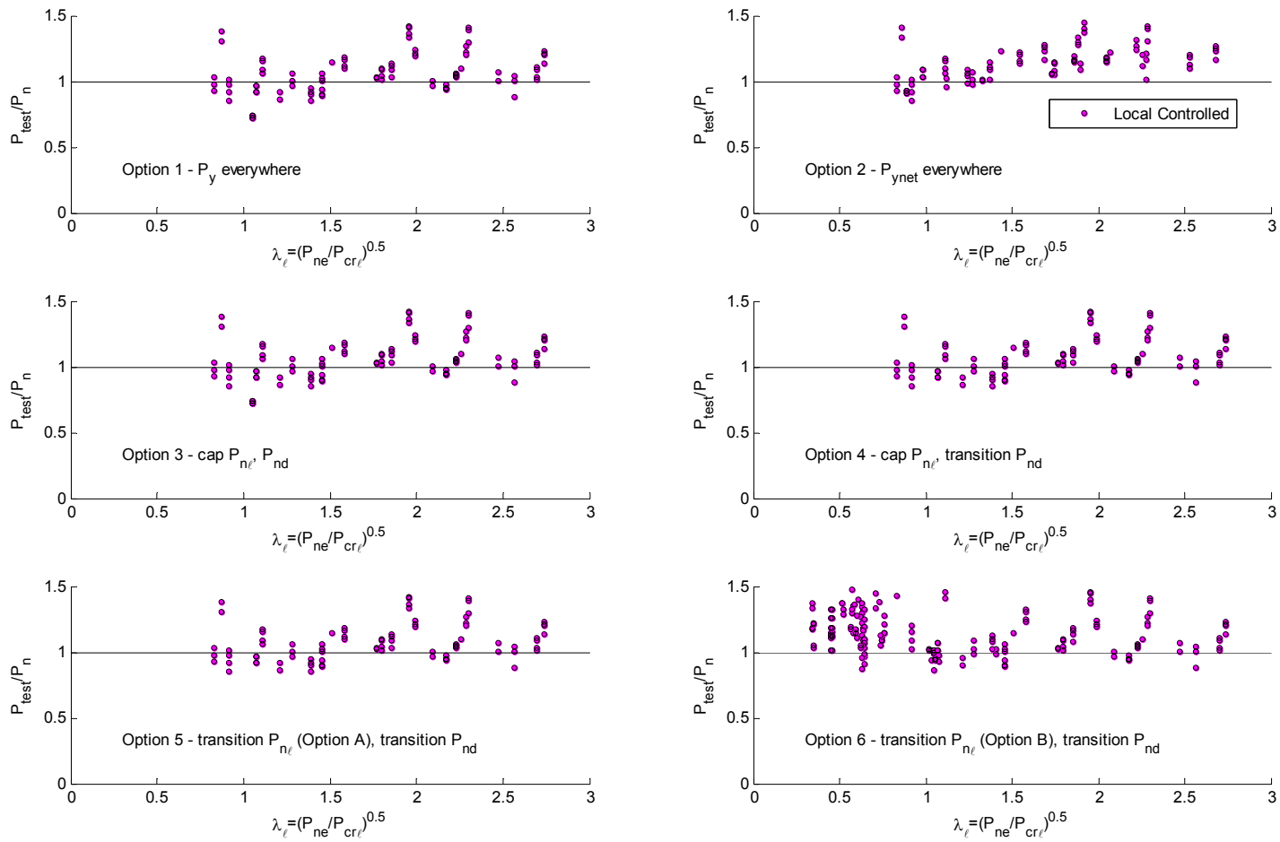
Figure 8.22 Test-to-predicted ratios for local buckling-controlled simulated column failures as a function of local slenderness
