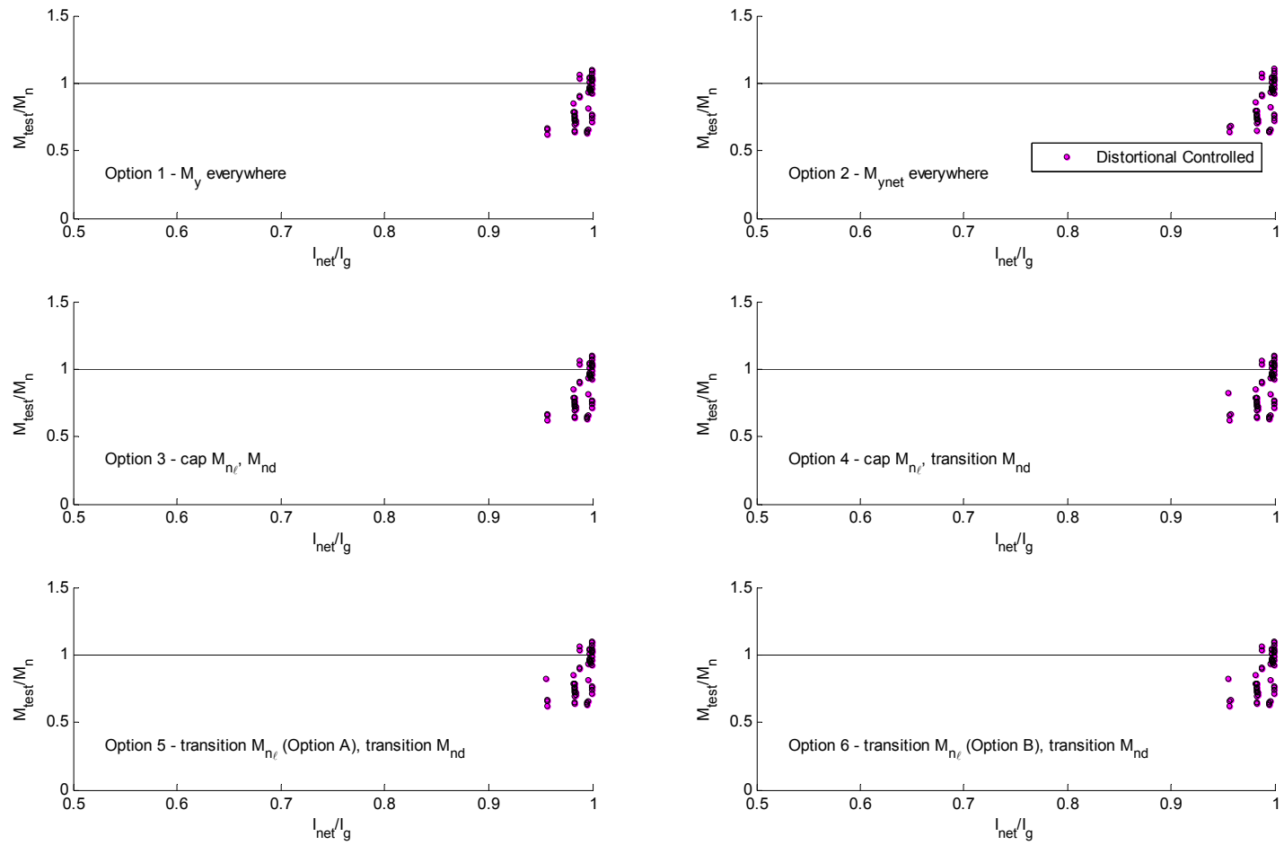
Figure 8.65 Test-to-predicted ratios for experimental distortional buckling-controlled laterally braced beam failures as a function of net cross-sectional moment of inertia to gross cross-sectional moment of inertia
