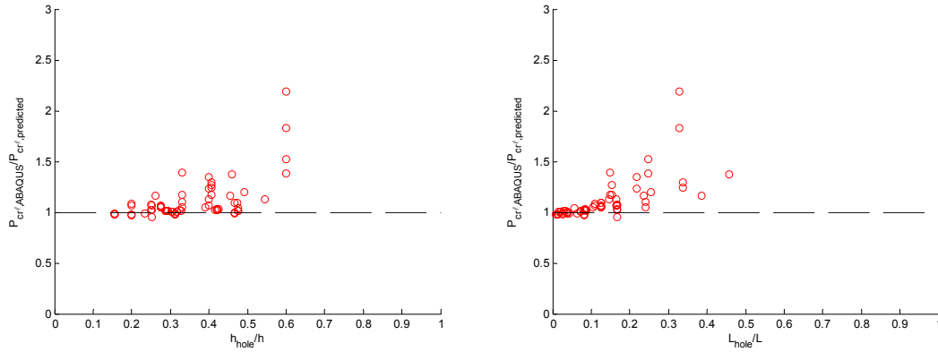
Figure 4.25 Predicted P_{cr\ell} (CUFSM approximate method) is compared relative to the ABAQUS P_{cr\ell} with experiment boundary conditions as a function of (a) hole width to flat web width and (b) hole length to column length
