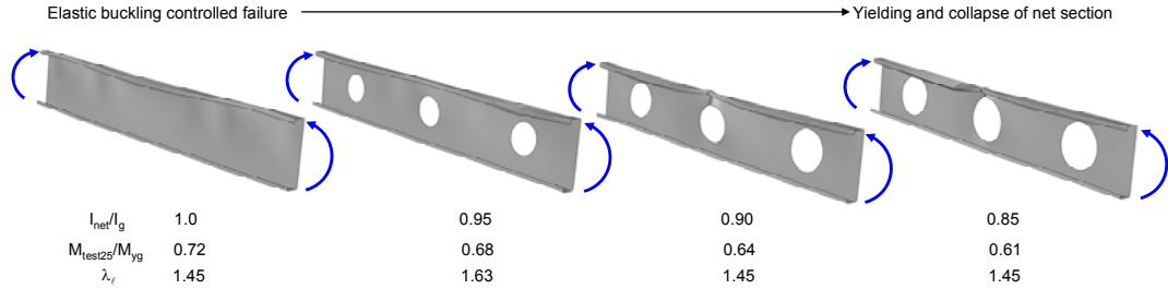
Figure 8.45 SSMA 800S162-43 beam with web holes considered in the DSM local buckling study
