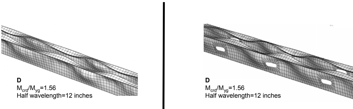
Figure 4.63 Distortional buckling modes for specimen 6B,18,1&2(H) with and without holes
