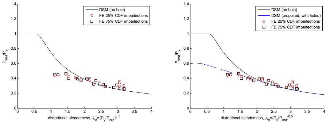
Figure 8.8 Comparison of simulated column strengths ( A_{net}/A_g=0.60 ) to (a) the existing DSM distortional buckling design curve and to (b) the proposed DSM distortional buckling curve for columns with holes
