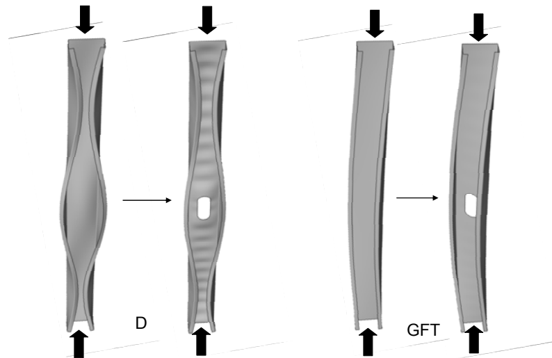
Figure 4.7 Influence of a slotted hole on the (a) distortional (D) and (b) global flexural-torsional (GFT) modes of a cold-formed steel column
