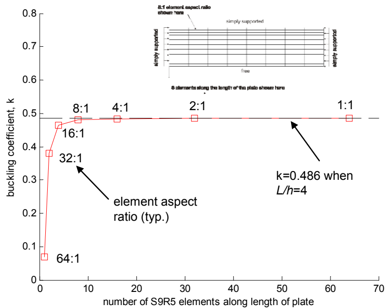
Figure 2.6 Accuracy of S9R5 elements as the number of finite elements provided along an unstiffened element varies, L/h=4
