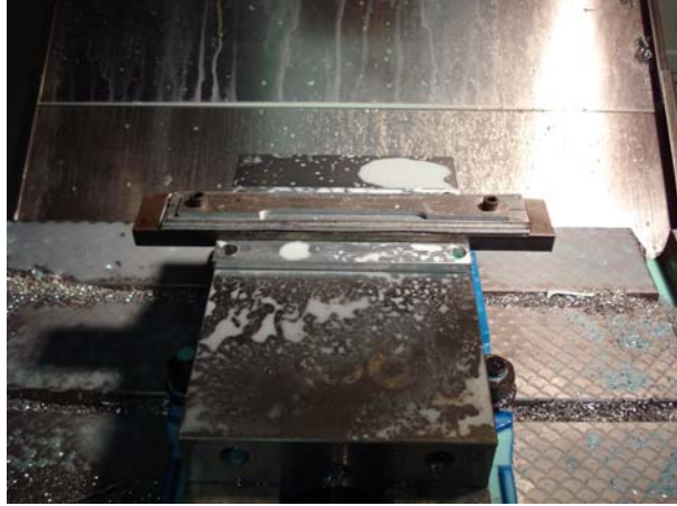
Figure 5.28 A custom jig allows three tensile coupons to be milled at once in the CNC machine
