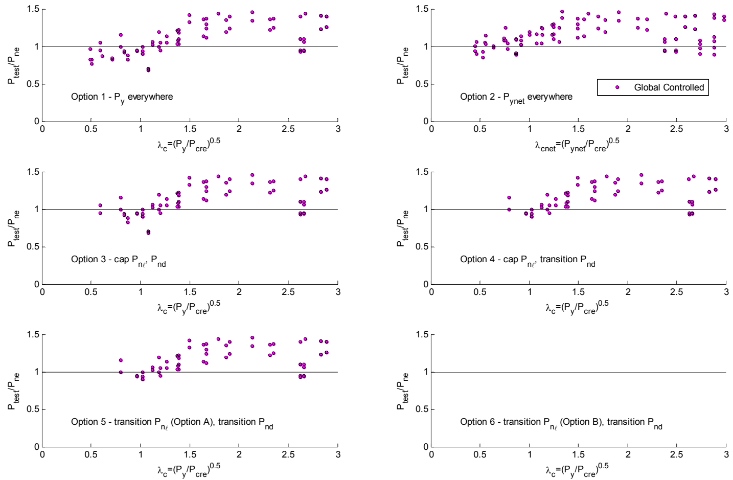
Figure 8.24 Test-to-predicted ratios for simulated global buckling-controlled column failures (i.e., no local buckling interaction) as a function of global slenderness
