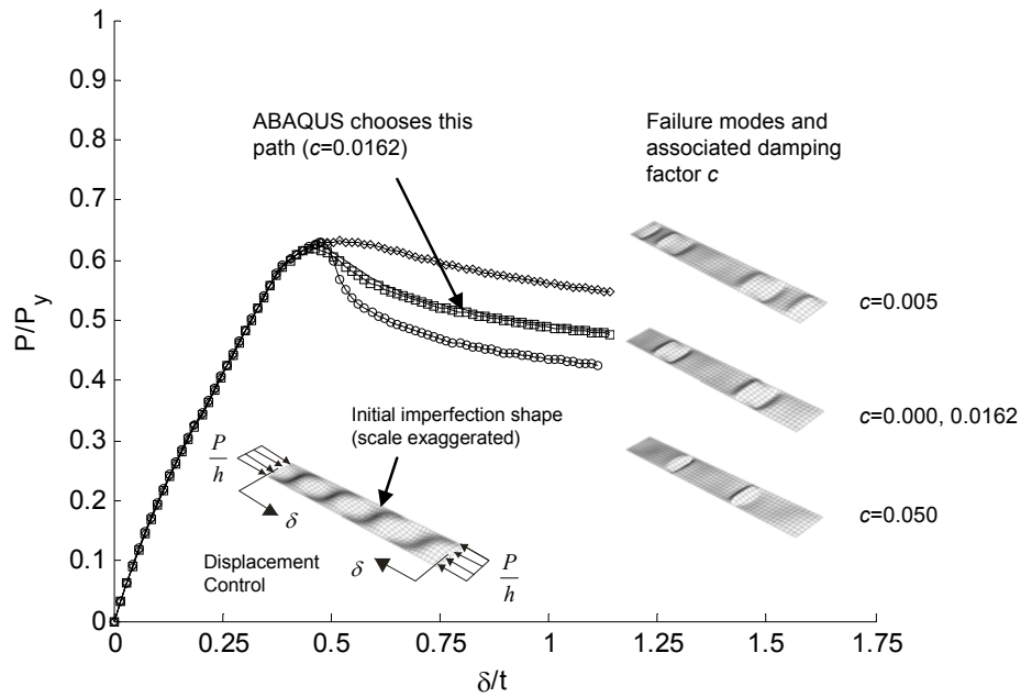
Figure 7.7 Artificial damping load-displacement solutions and failure modes
