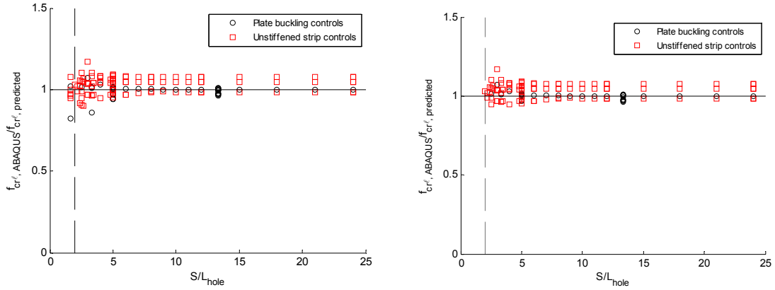
Figure 3.16 Accuracy of stiffened element prediction method as a function of hole spacing S to length of hole L_{hole} (a) without and (b) with the dimensional limits in Eq. (3.8) and Eq.(3.9)
