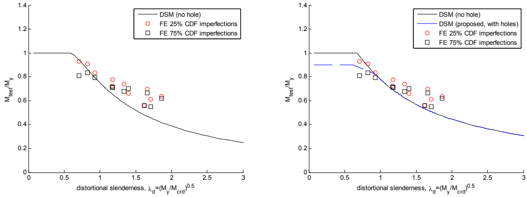
Figure 8.53 Comparison of simulated beam strengths ( I_{net}/I_g=0.90 ) to (a) the existing DSM distortional buckling design curve and to (b) the proposed DSM distortional buckling curve for beams with holes
