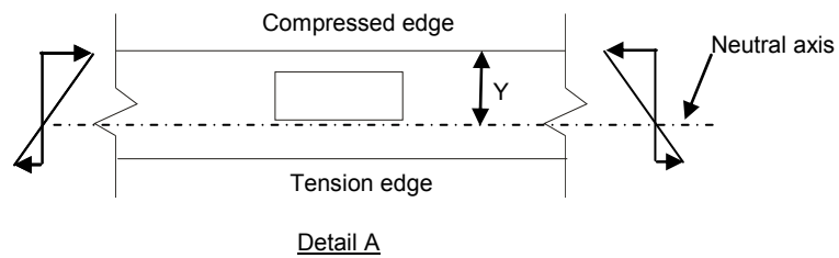
Figure 3.4 Definition of neutral axis location for stiffened elements in bending.
