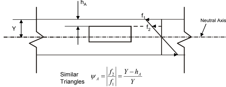
Figure 3.30 Derivation of stress ratio \psi_A for unstiffened strip "A".
