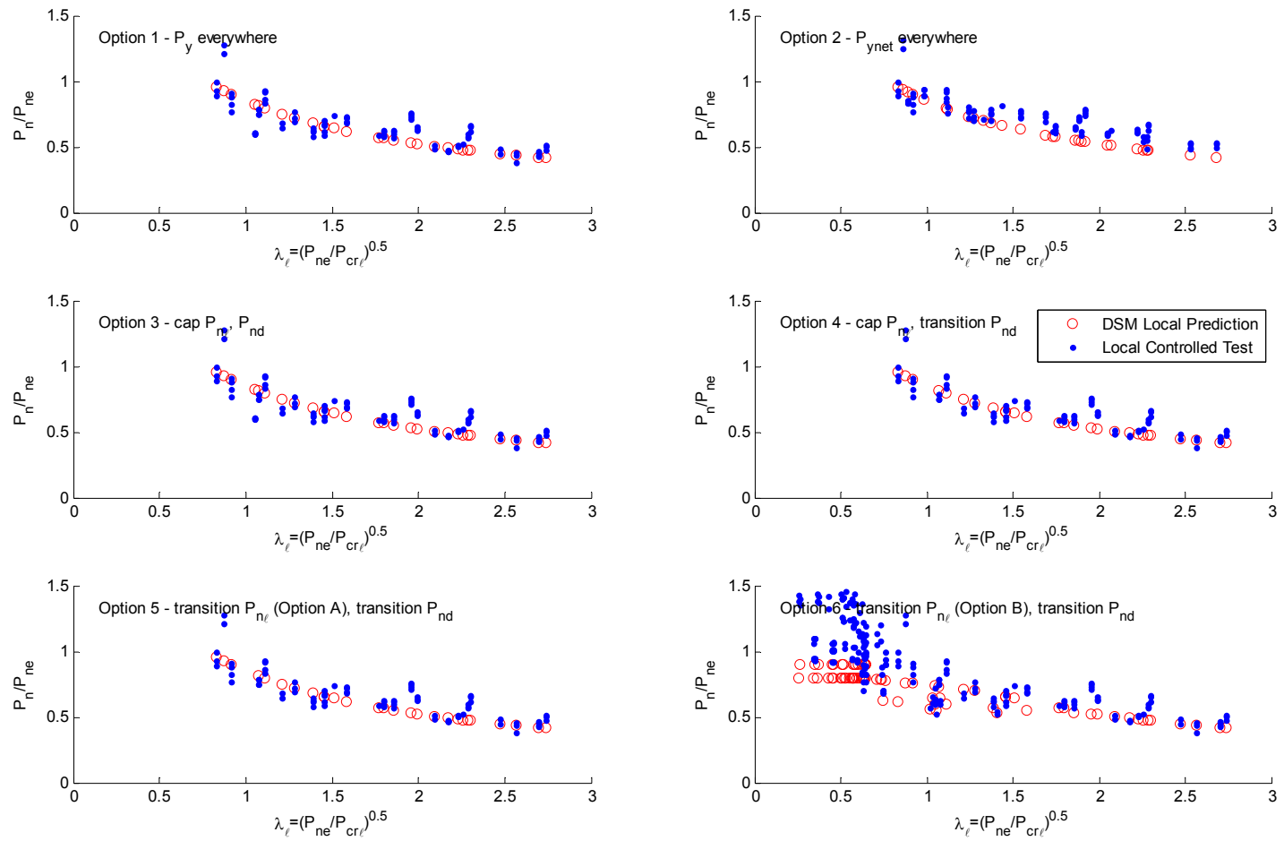
Figure 8.18 Comparison of simulated test strengths to predictions for columns with local buckling-controlled failures as a function of local slenderness (tested strength is normalized by P_{ne} )
