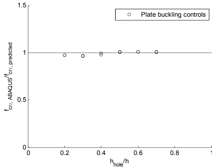
Figure 3.20 Accuracy of prediction method for stiffened elements with square or circular holes as a function of hole width h_{\text{hole}} to plate width h .
