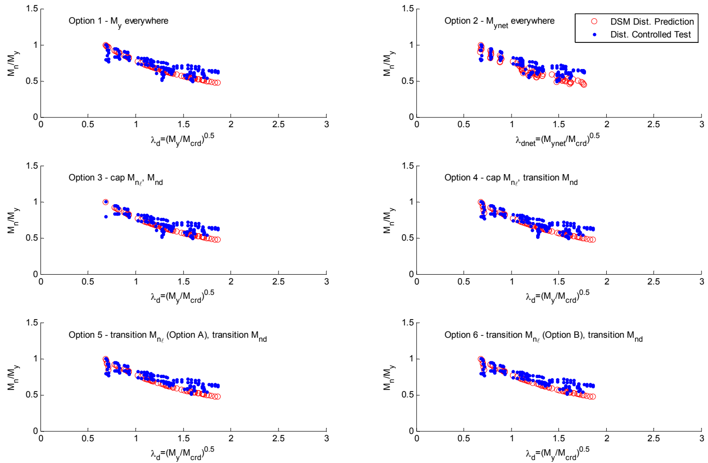
Figure 8.55 Comparison of simulated test strengths to predictions for laterally braced beams with distortional buckling-controlled failures as a function of distortional slenderness
