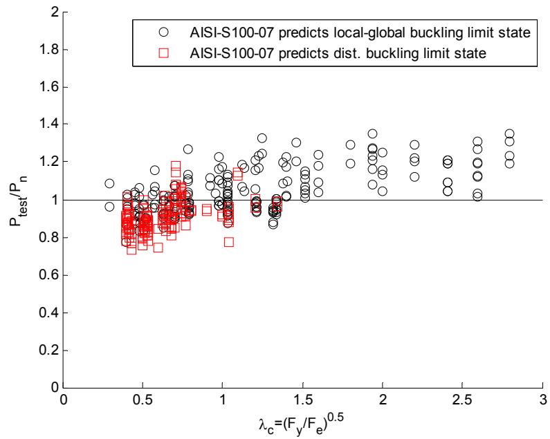
Figure M.2 AISI S100-07 test-to-predicted ratio for FE simulated tests of columns with holes
