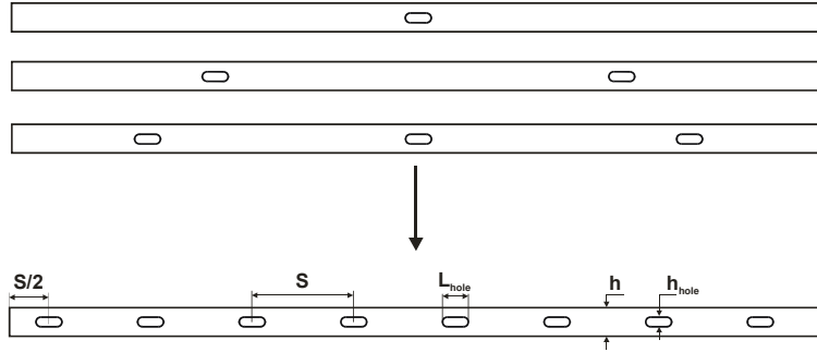
Figure 3.10 Definition of center-to-center dimension for the slotted holes
