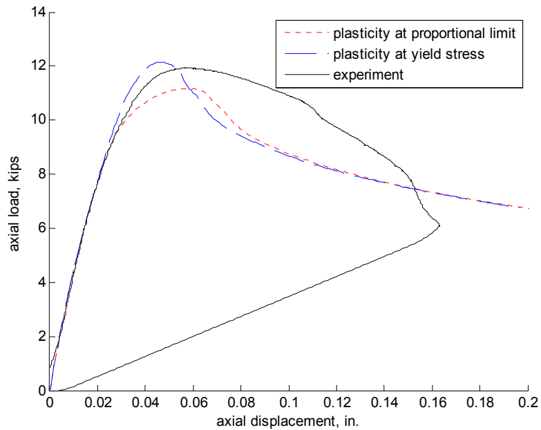
Figure 7.30 Influence of ABAQUS material model on the load-deformation response of specimen 600-1-24-NH (work this figure with Figure 7.29)
