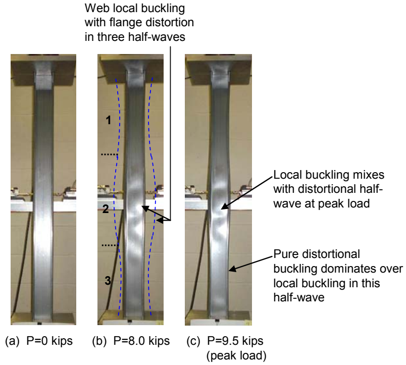
Figure 5.44 Load-displacement progression, intermediate length column specimen 362-3-48-NH
