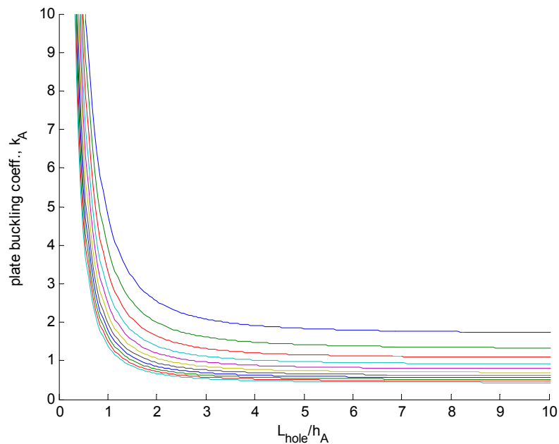
Figure C.2 The plate buckling coefficient k_A for an unstiffened element in compression (the multiple curves represent 0 \leq \psi_A \leq 1 with a step of 0.1, 11 curves total)
