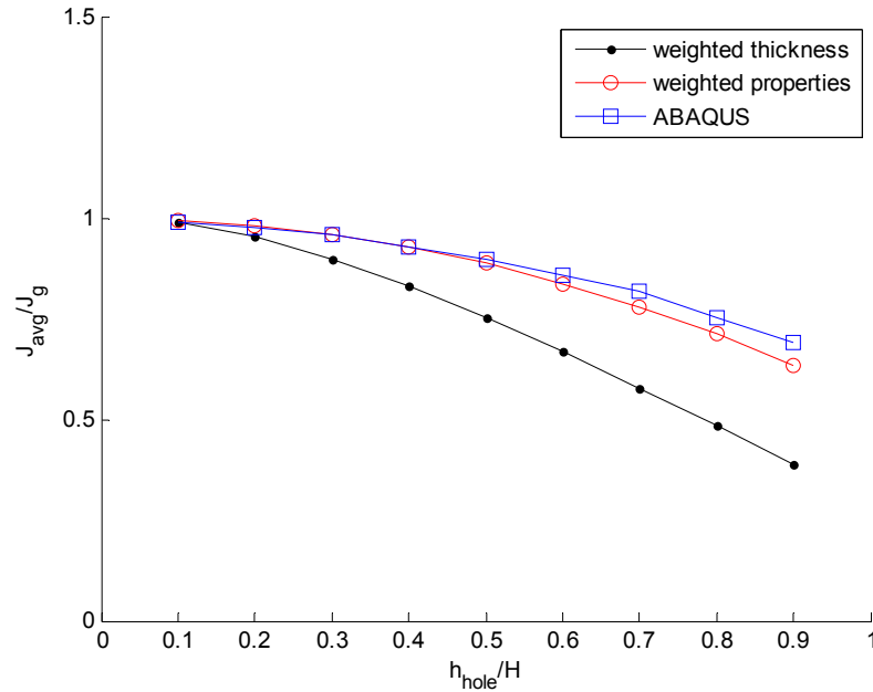
Figure 4.43 The “weighted properties” approximation for J_{avg} matches closely with the ABAQUS prediction for the SSMA 12S00162-68 column with holes
