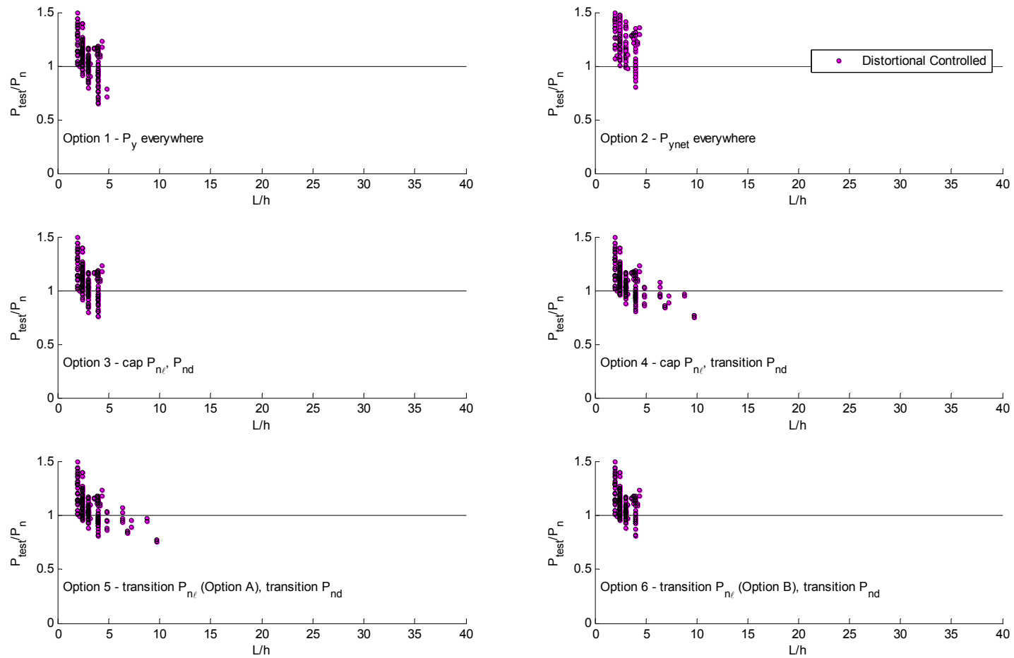
Figure 8.29 Test-to-predicted ratios for simulated distortional buckling-controlled column failures as a function of column length, L , to flat web width, h
