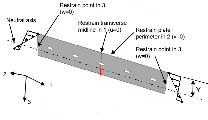
Figure 3.24 Boundary and loading conditions for a stiffened element in bending
