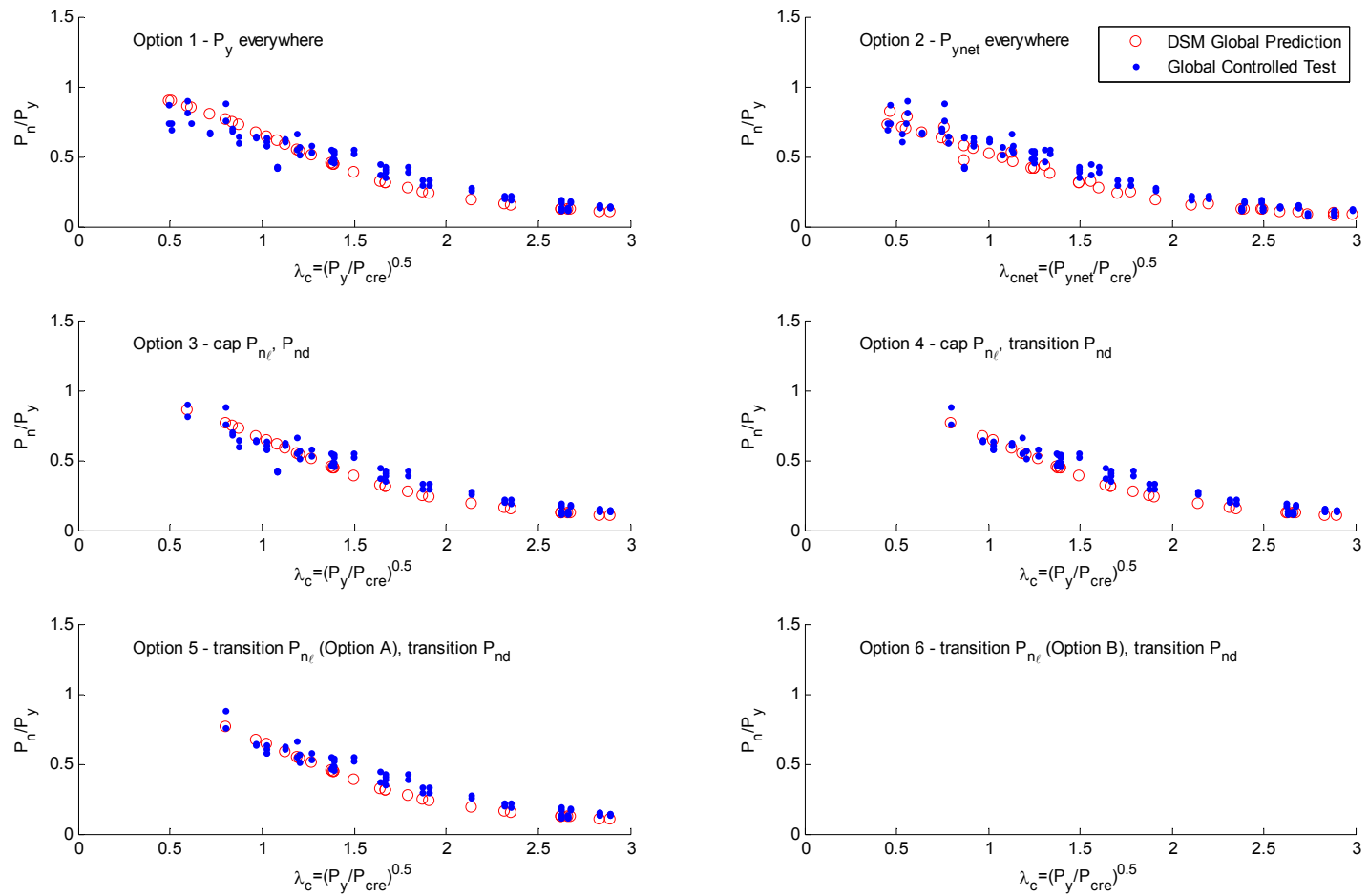
Figure 8.21 Comparison of simulated test strengths to predictions for columns with global buckling-controlled failures (i.e., no local interaction) as a function of global slenderness
