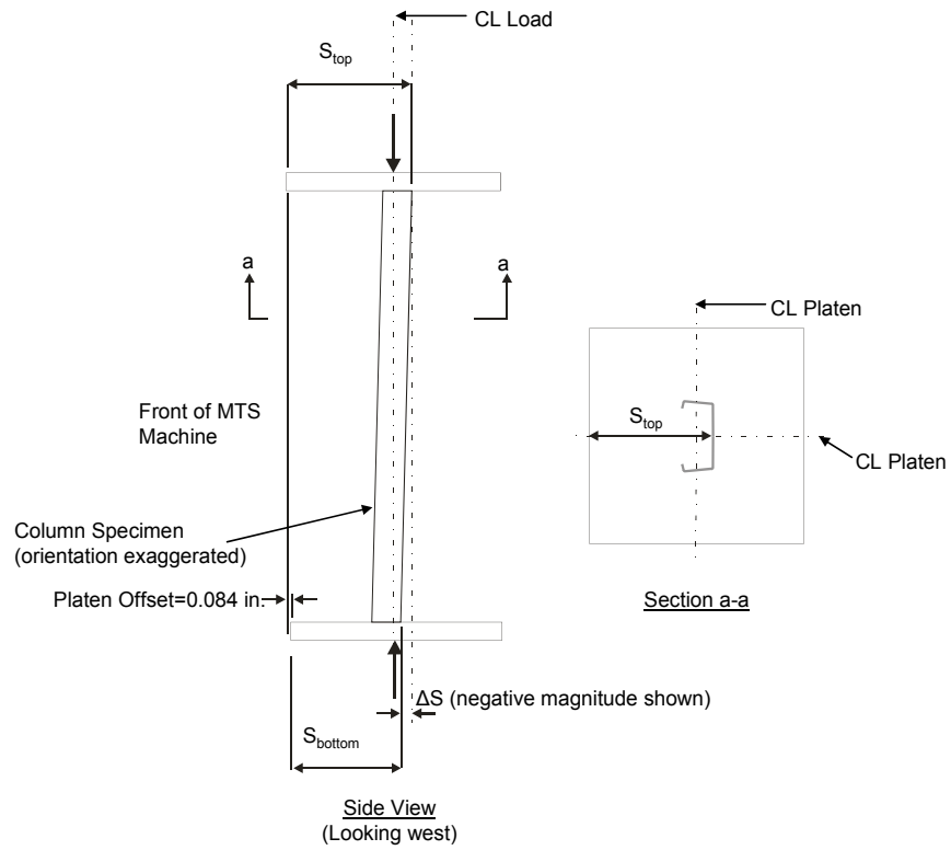
Figure 5.24 Column specimen weak axis out-of-straightness schematic
