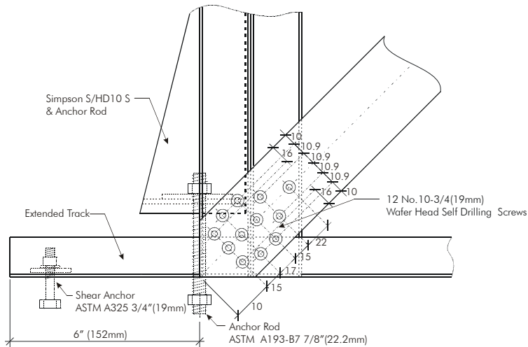
Figure 2.16 Nominal dimensions and the corner detail of specimens 35A-M and 36A-C
