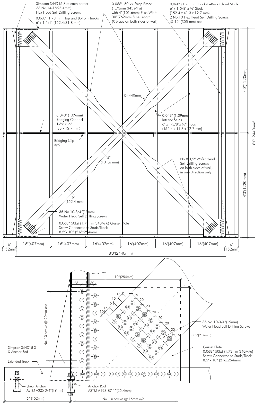
Figure 2.32 Nominal dimensions and corner detail of specimens 29A-M 2 and 30A-C
