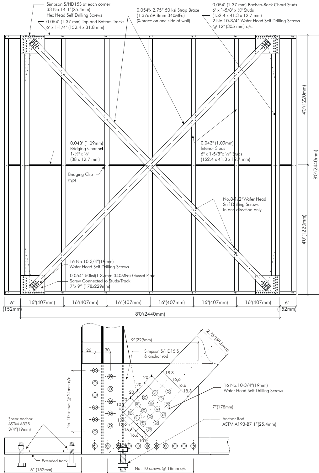
Figure 2.25 Nominal dimensions and the corner detail of specimens 47A-M and 48A-C
