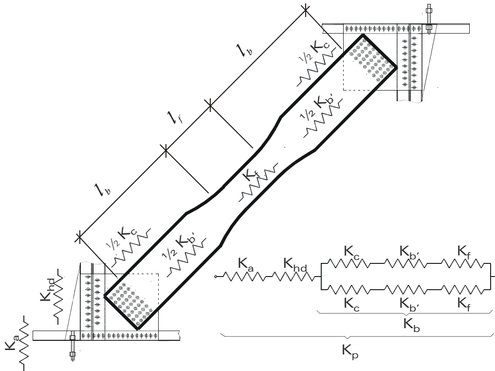
Figure 2.48 Model for the predicted stiffness
