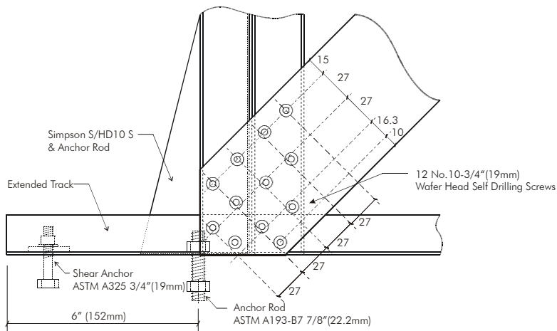
Figure 2.14 Nominal dimensions and the corner detail of specimens 25A-M and 26A-C
