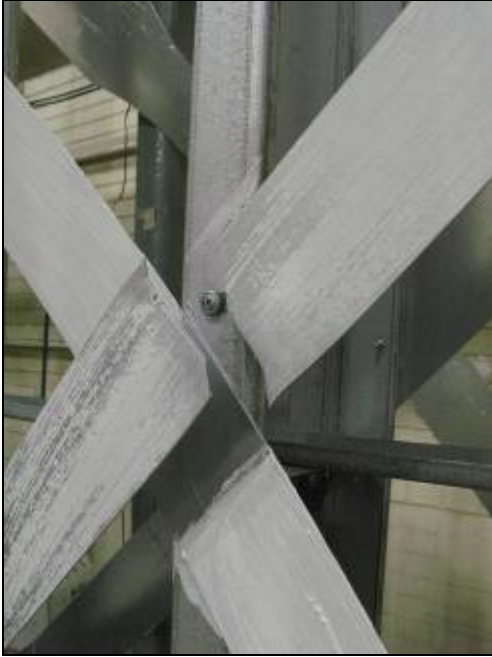
Figure 2.54 Net section fracture of braces of specimen 27A-M 2 at 3.6% drift
