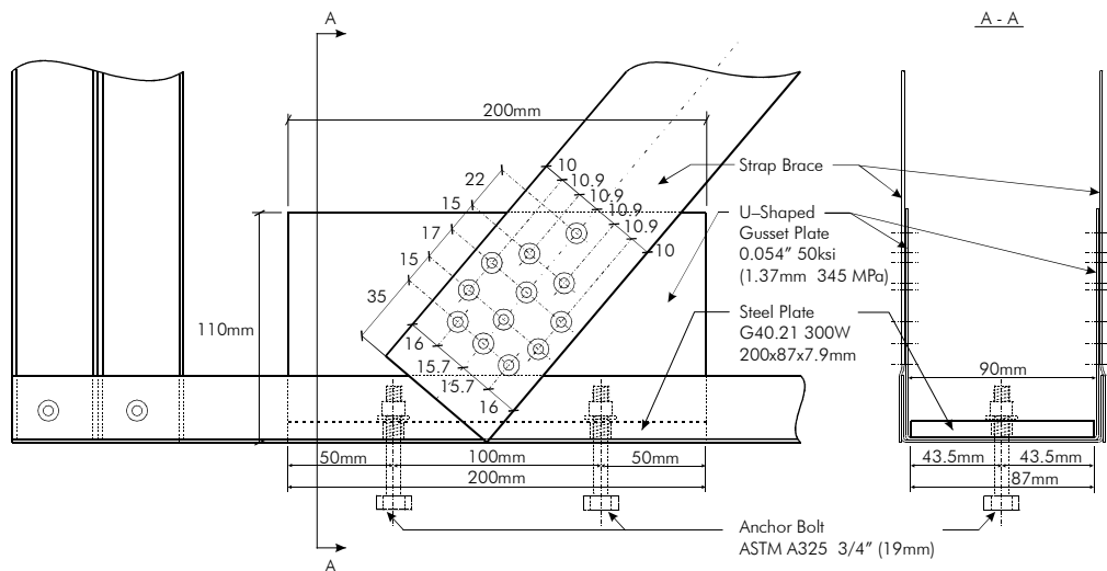
Figure 2.17 Nominal dimensions and the corner detail of specimens 41 A-M and 42 A-C
