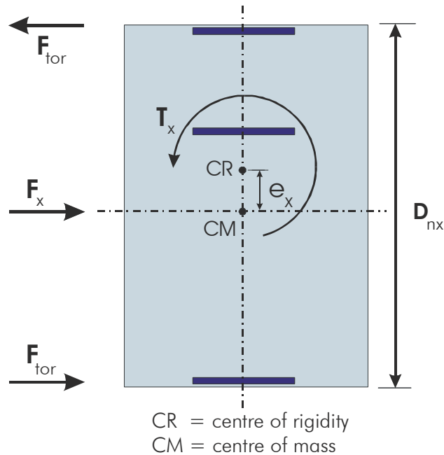
Figure 3.5 Torsional effects
