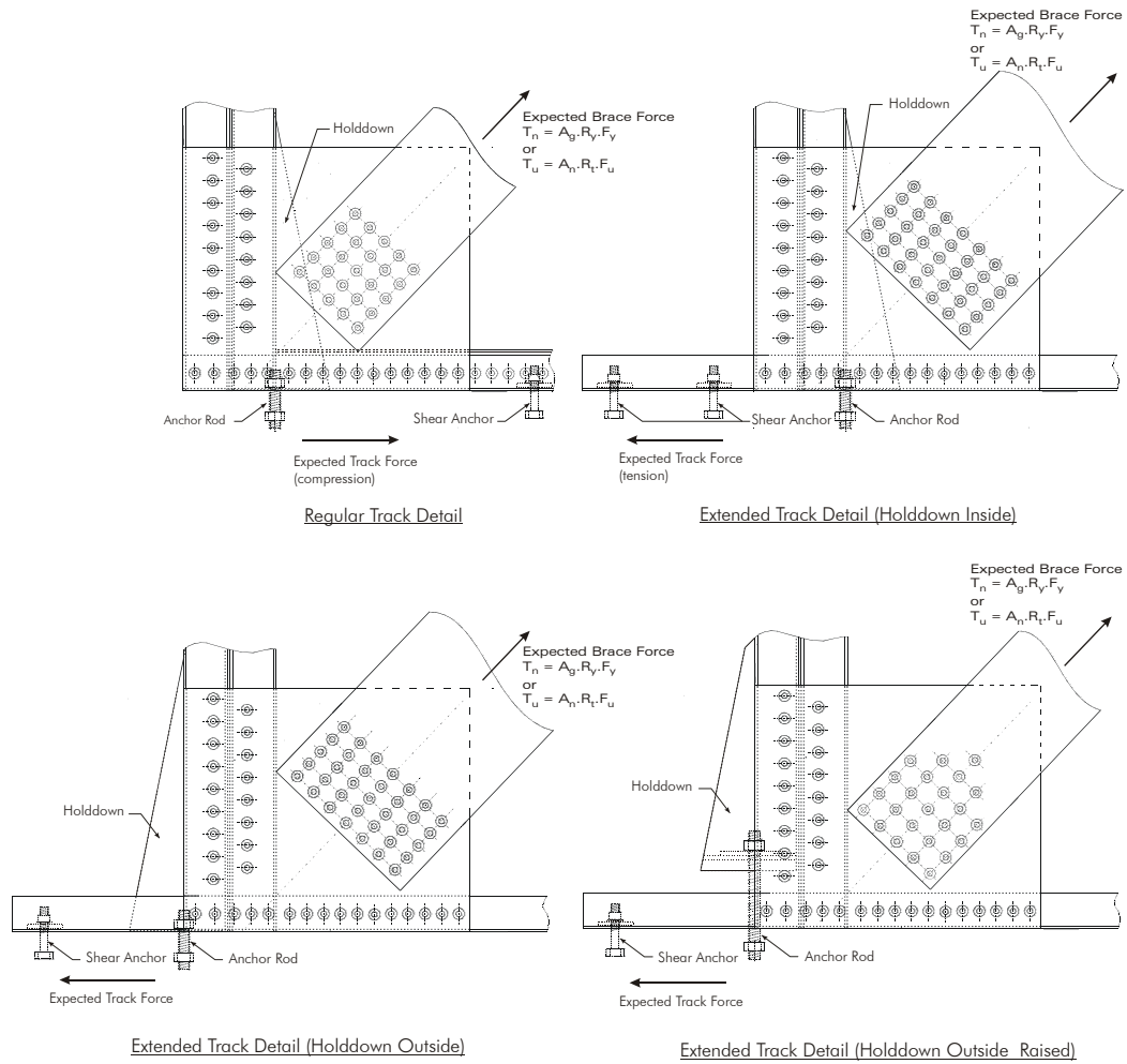
Figure 2.12 Track details showing track force
