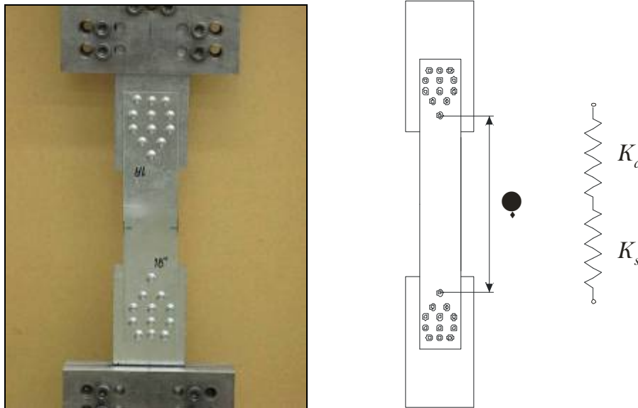
Figure 2.49 Connection test
