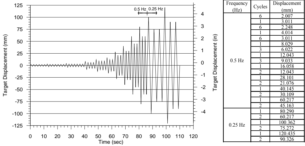
Figure A.20 Reversed cyclic CUREE test protocol for specimen 34A-C
