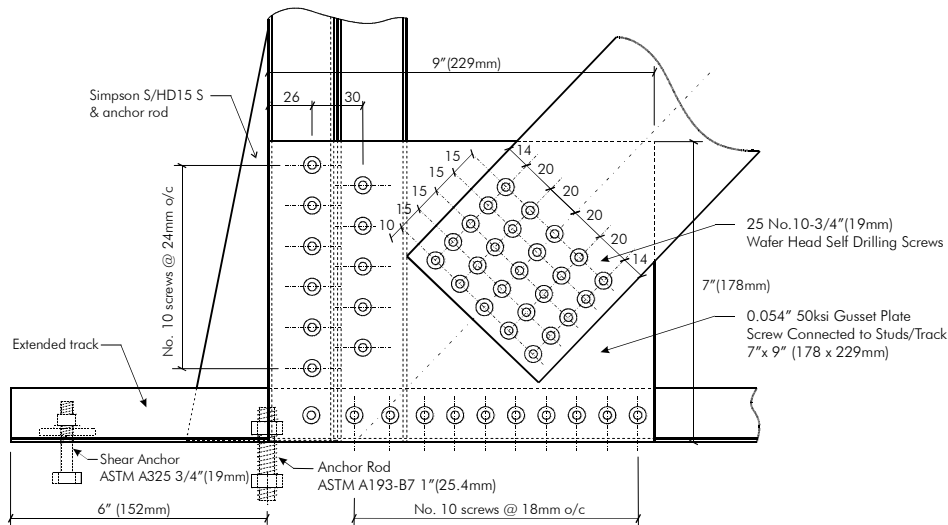
Figure 2.23 Nominal dimensions the corner detail of specimens 27A-M and 28A-C
