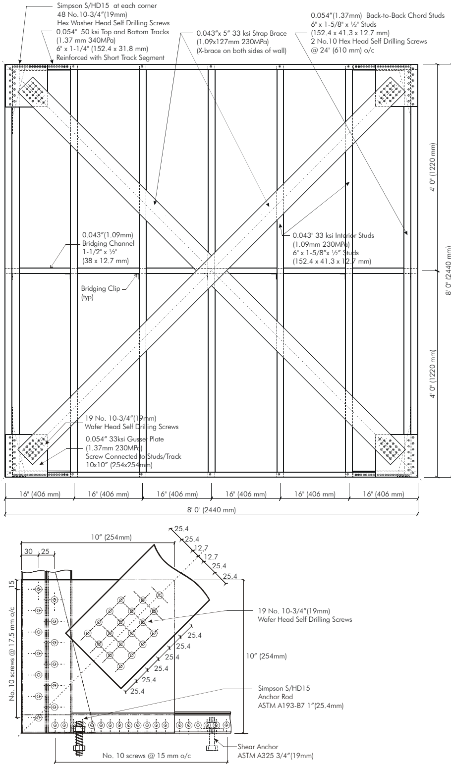
Figure 2.22 Nominal dimensions and the corner detail of specimen 9C-M
