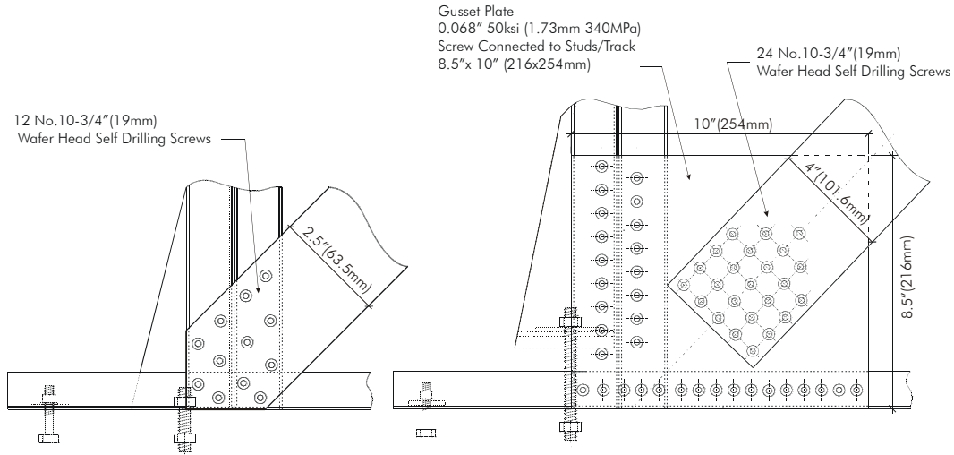
Figure 2.6 Corner details light and medium walls
