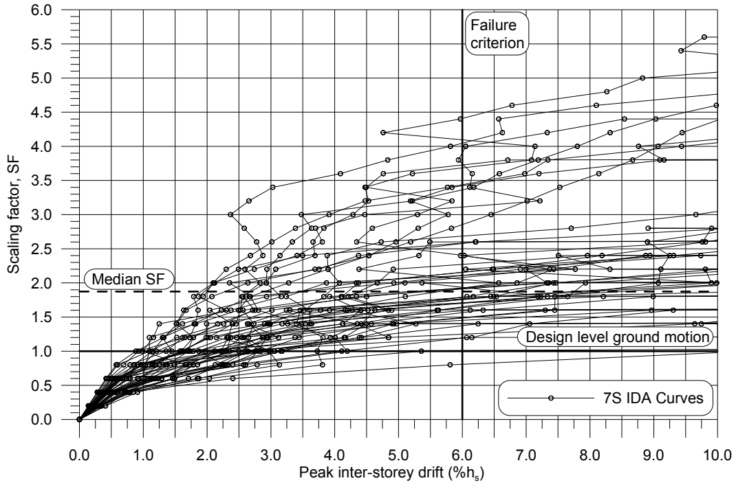
Figure I.19: IDA analysis for model 7S R_dR_o4 -minbrace
