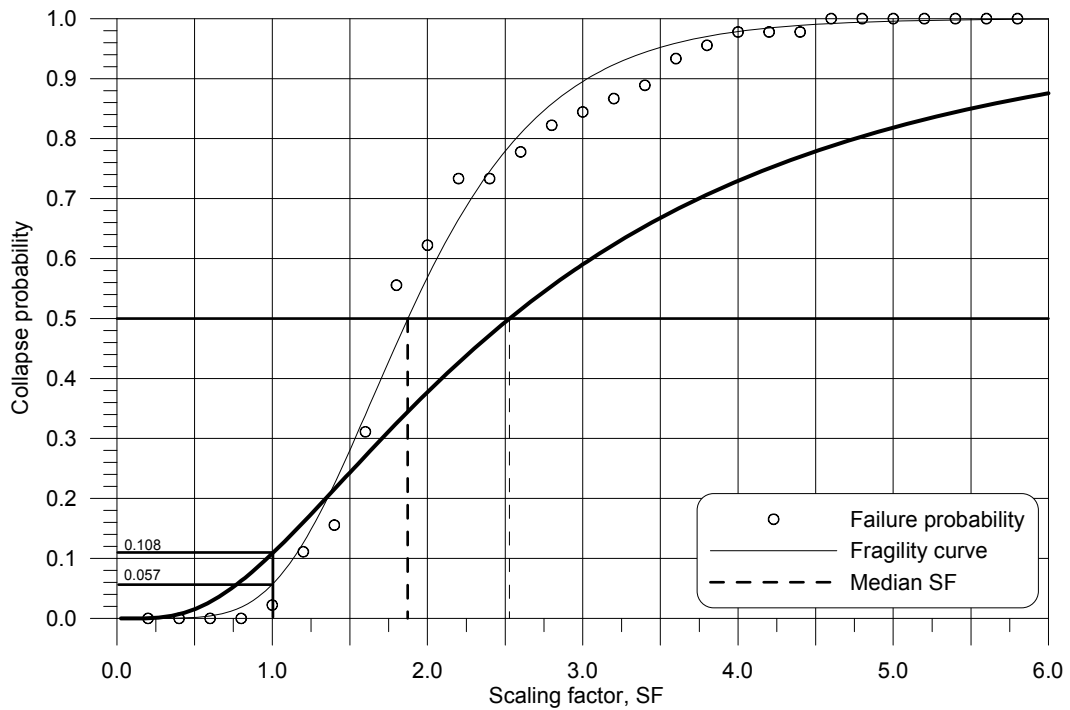
Figure I.20: Fragility curve for model 7S R_dR_o4 -minbrace
