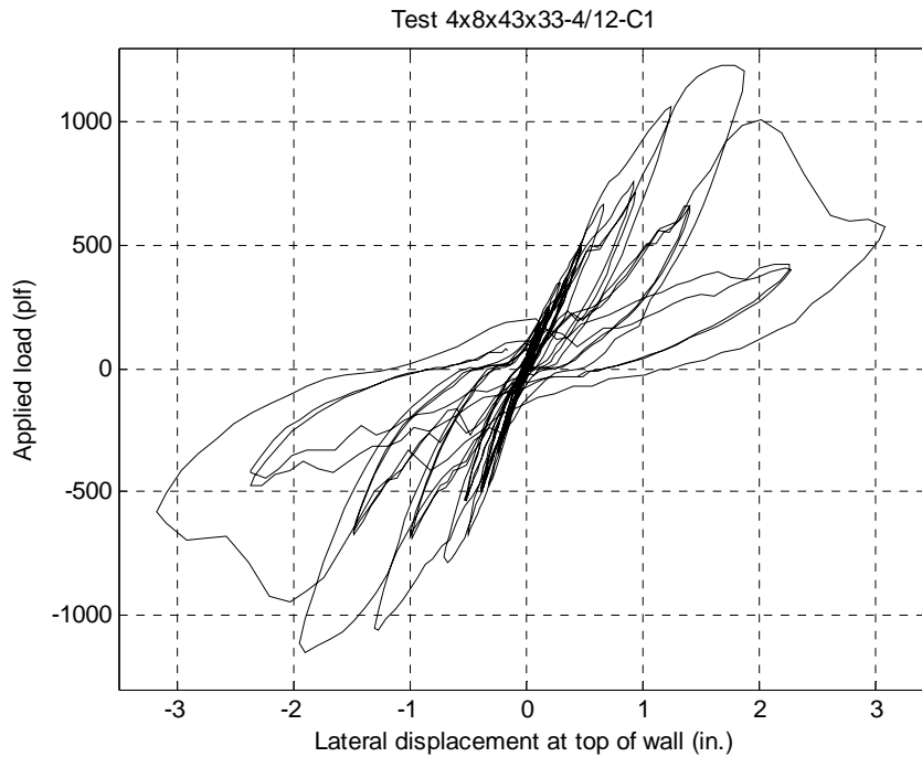
Figure 16 Observed hysteresis curve for test 4×8×43×33-4/12-C1
