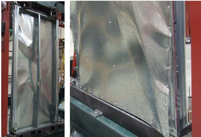
Figure 17 Failure mode for test 4×8×43×33-4/12-C1
