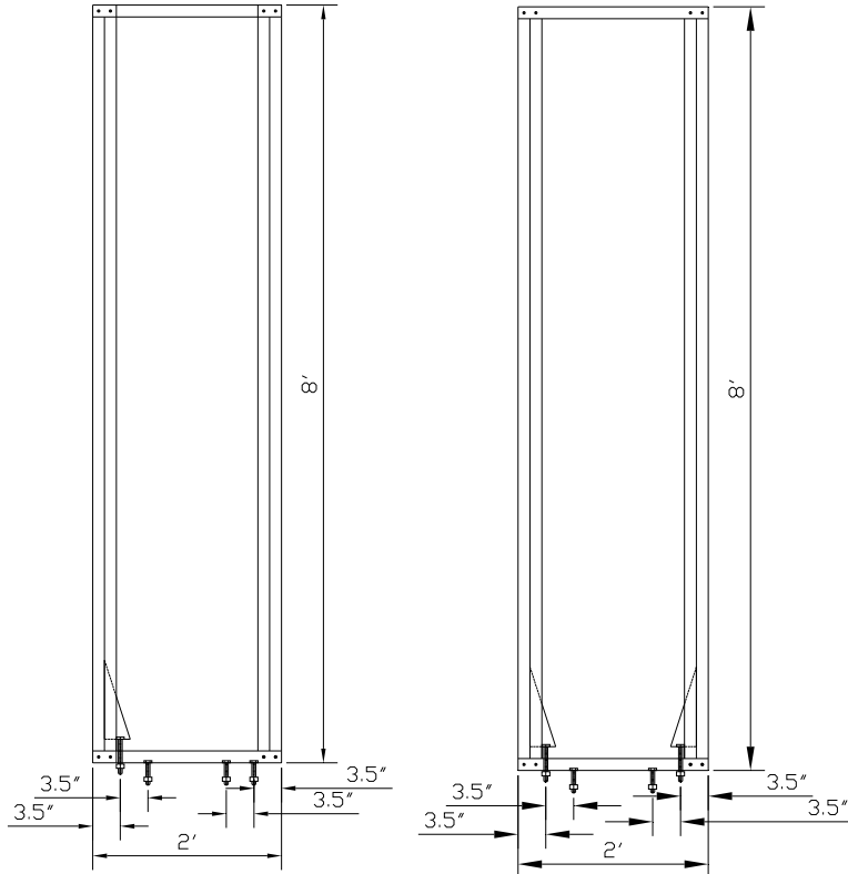
(a) wall assembly for monotonic test (b) wall assembly for cyclic test Figure 7 Dimensions of 8-ft. x 2-ft. wall assembly
