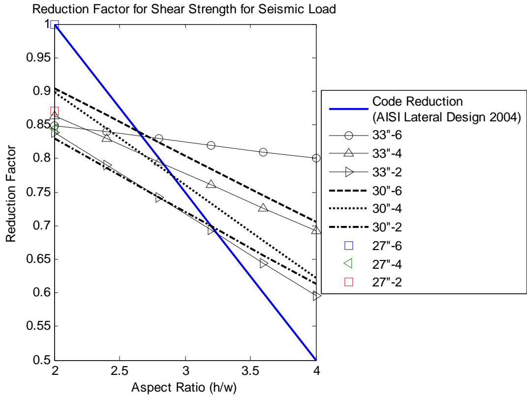
Figure 34 Reduction factors for shear strength for seismic loads
