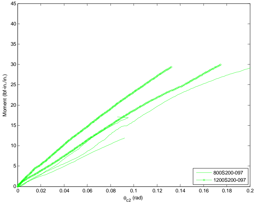
Figure 37 Influence of joist depth on connector response for 800S200-097 and 1200S200-097 joists
