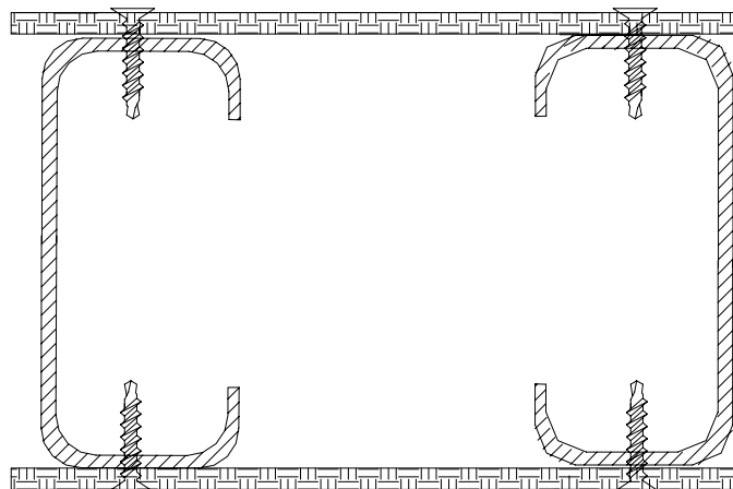
Figure 12 - Section A-A
