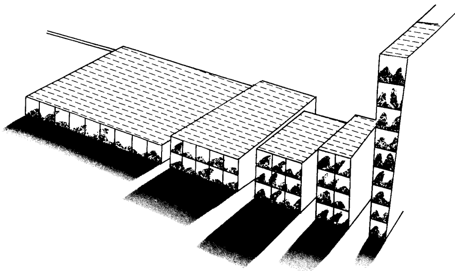
Figure 31. The effect of shape of exposing building face on distance separation. The five buildings have the same area of building face. The greater radiation intensity at a fixed distance for the more nearly square radiating wall is evident.
